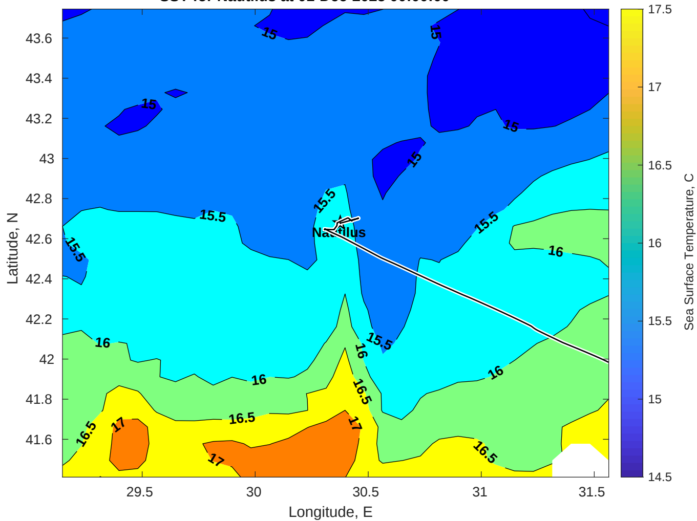
SST for Nautilus at 01-Dec-2025 00:00:00
