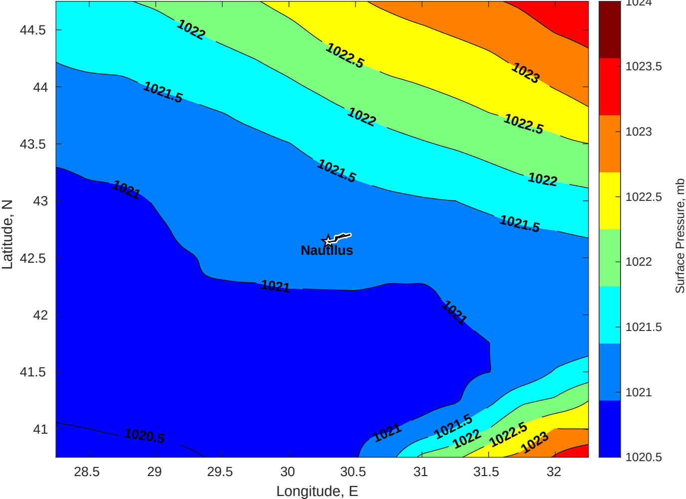
Surface Pressure (mb) for Nautilus at 04-Dec-2025 00:00:00
