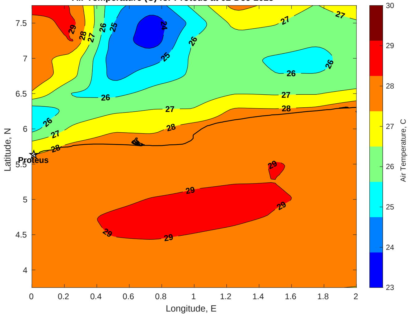
Air Temperature (C) for Proteus at 02-Dec-2025
