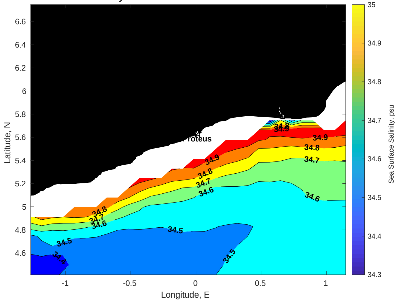
Surface Salinity for Proteus at 01-Dec-2025 00:00:00
