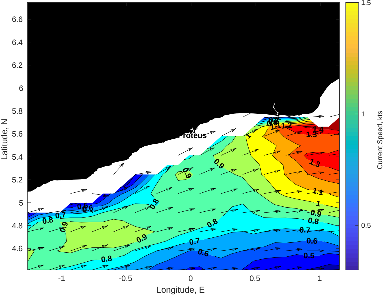
Surface Currents for Proteus at 01-Dec-2025 00:00:00
