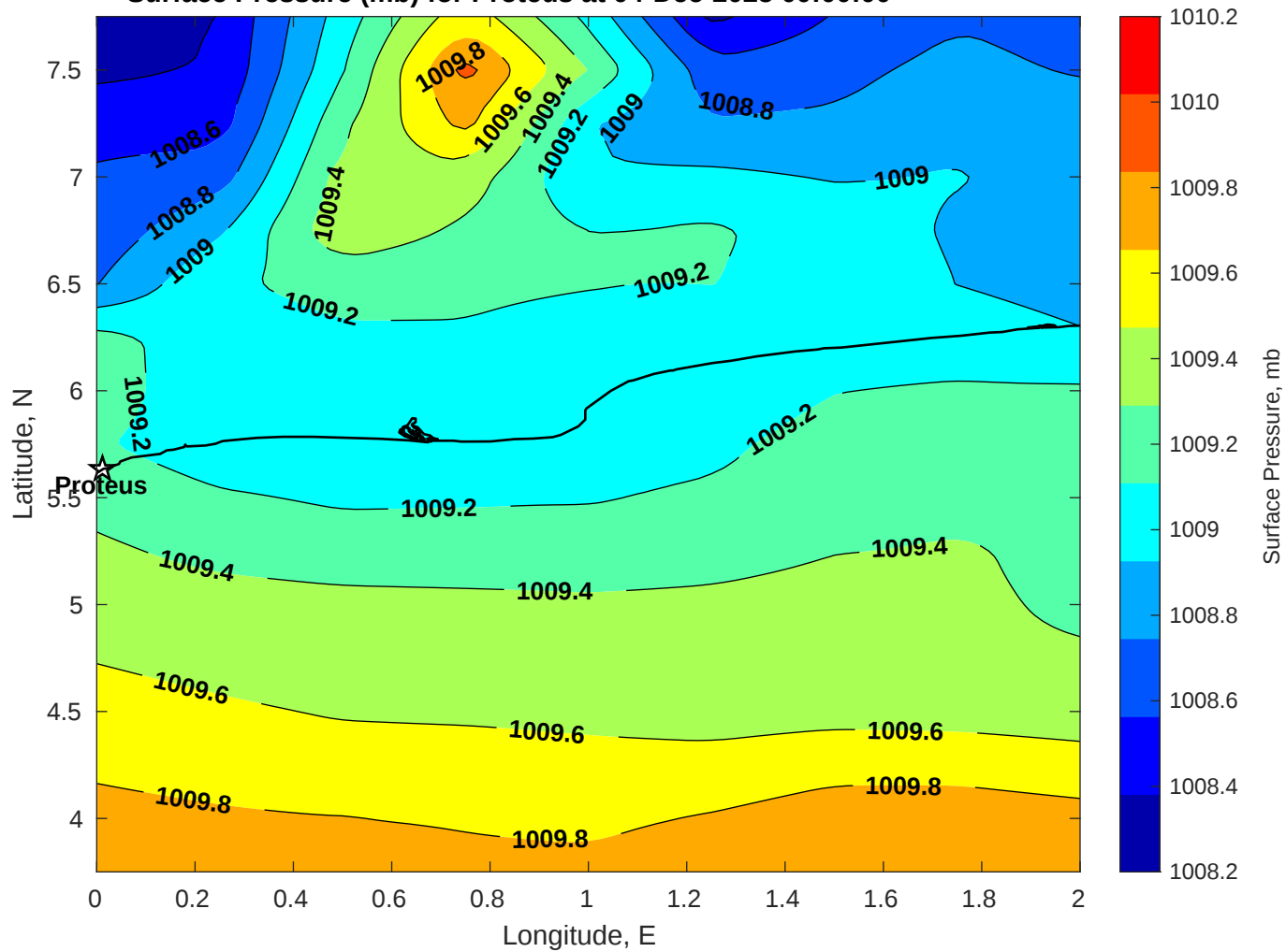
Surface Pressure (mb) for Proteus at 04-Dec-2025 00:00:00
