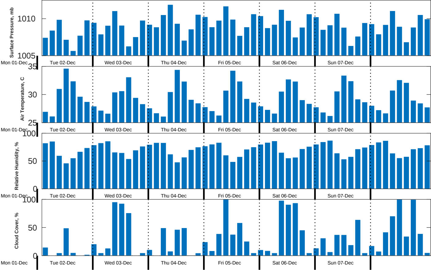
Met Forecast for Proteus from 02-Dec-2025 00:00:00 to 09-Dec-2025 00:00:00
