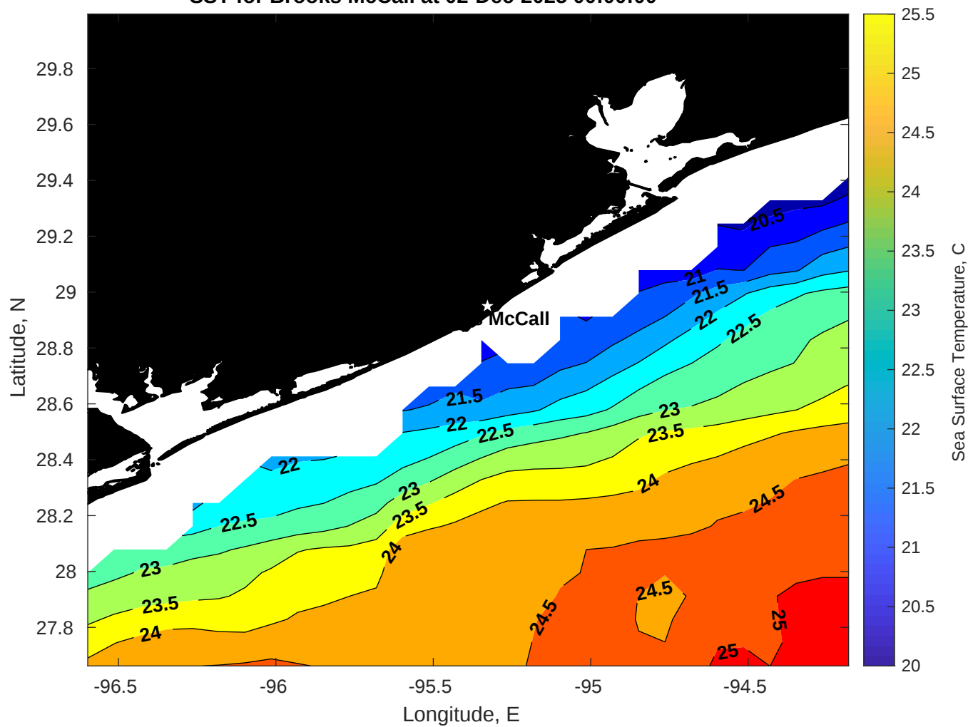
SST for Brooks McCall at 02-Dec-2025 00:00:00
