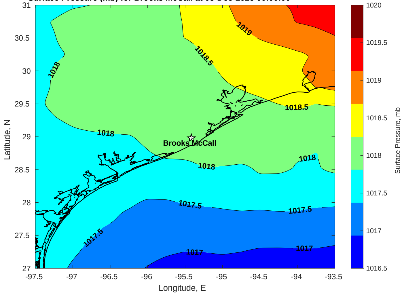
Surface Pressure (mb) for Brooks McCall at 03-Dec-2025 00:00:00
