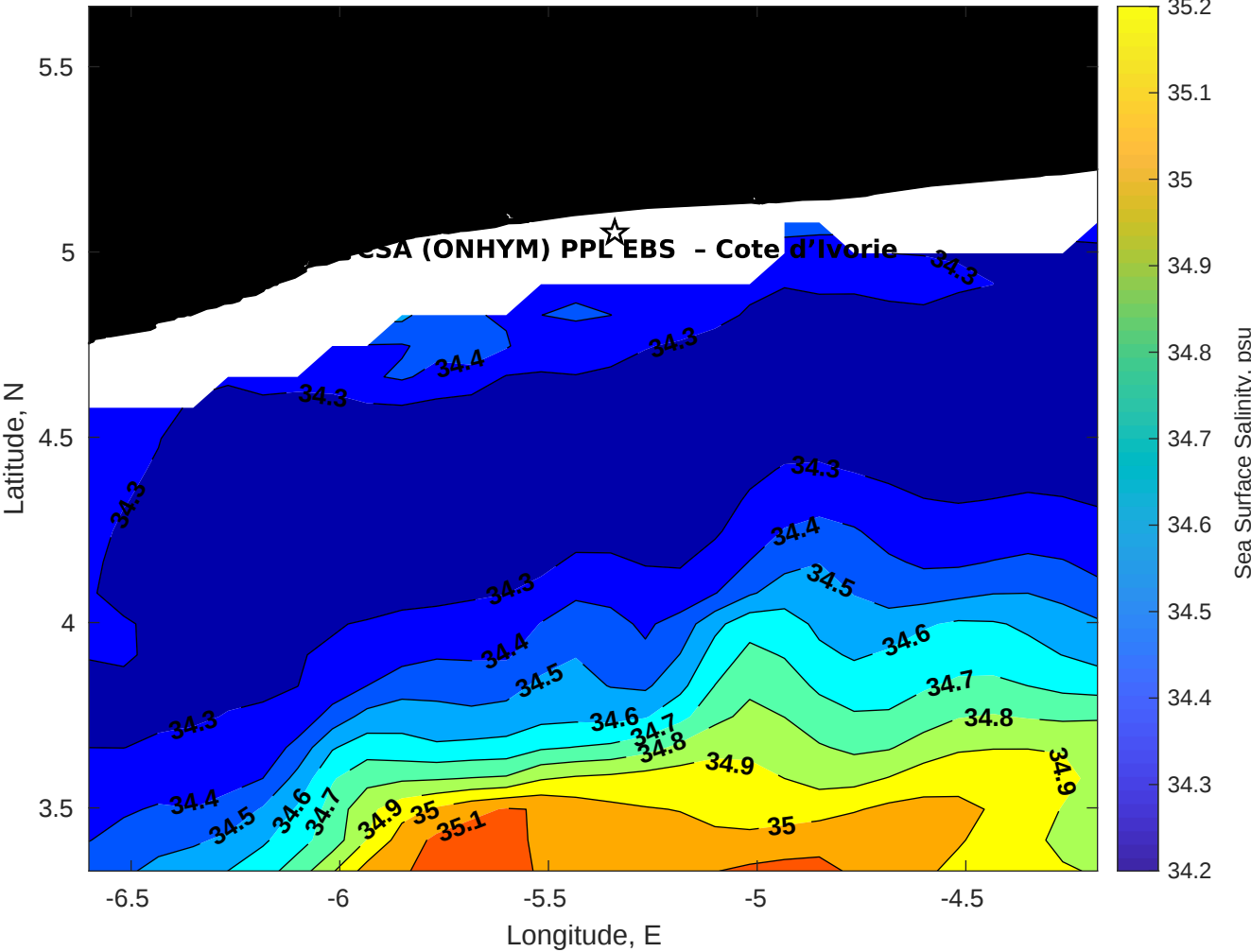
Surface Salinity for CSA (ONHYM) PPL EBS - Cote d'Ivoire at 02-Dec-2025 00:00:00
