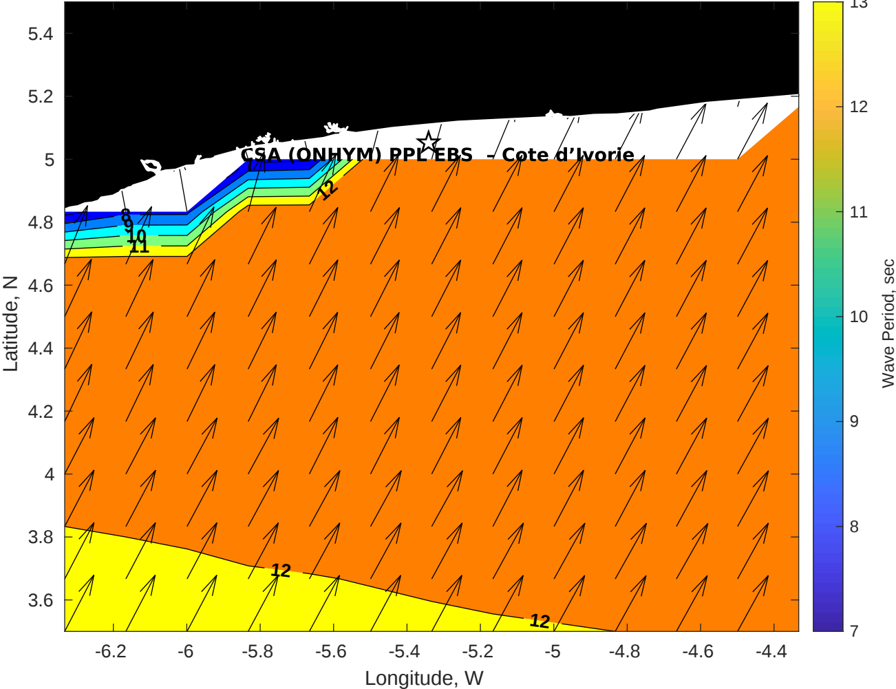
GFS Wave Period (sec) for CSA (ONHYM) PPL EBS - Cote d'Ivoire at 03-Dec-2025 09:00:00
