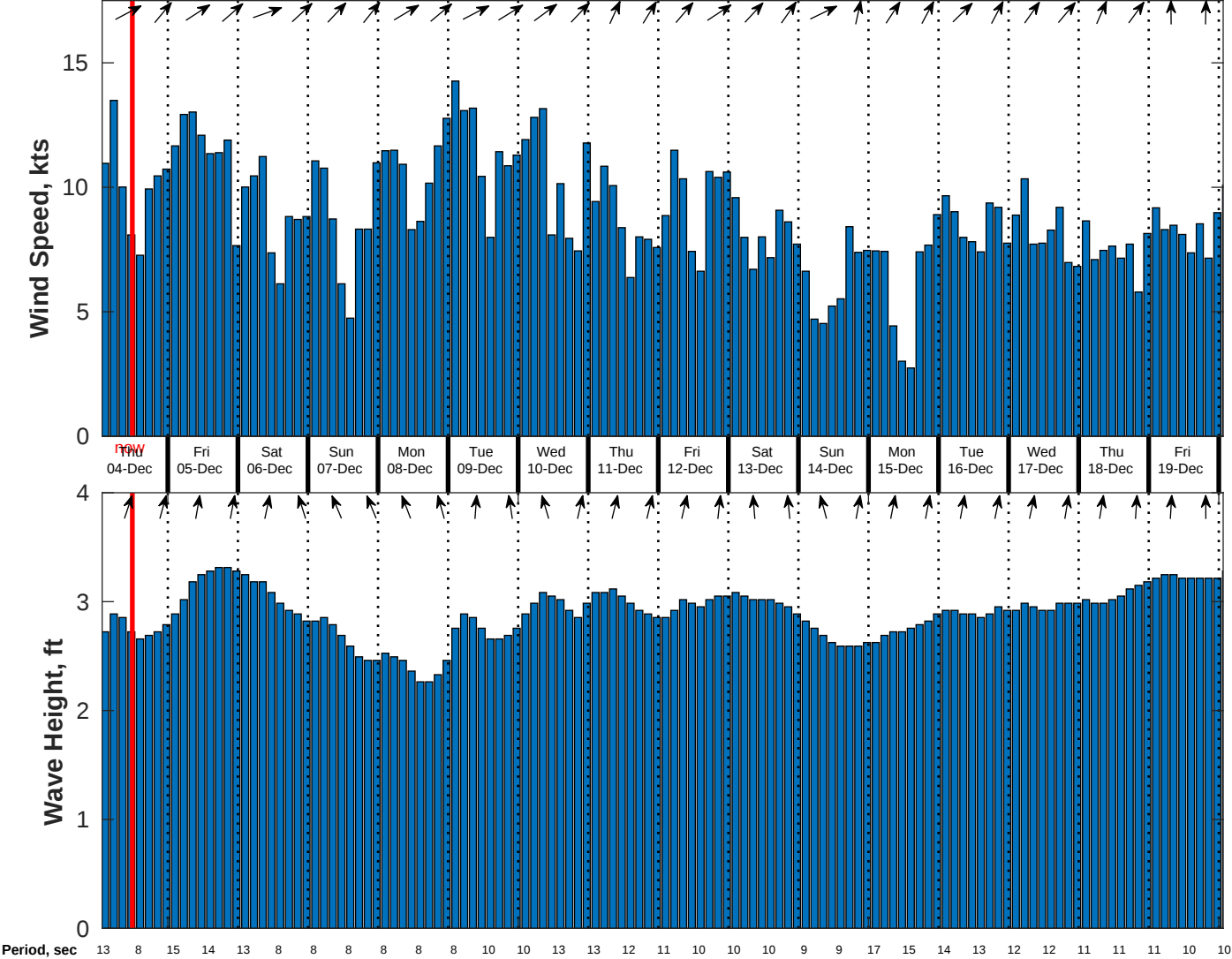
Wind & Wave Forecast for CSA (ONHYM) PPL EBS - Cote d'Ivoire from 03-Dec-2025 01:00:00 to 19-Dec-2025 01:00:00
