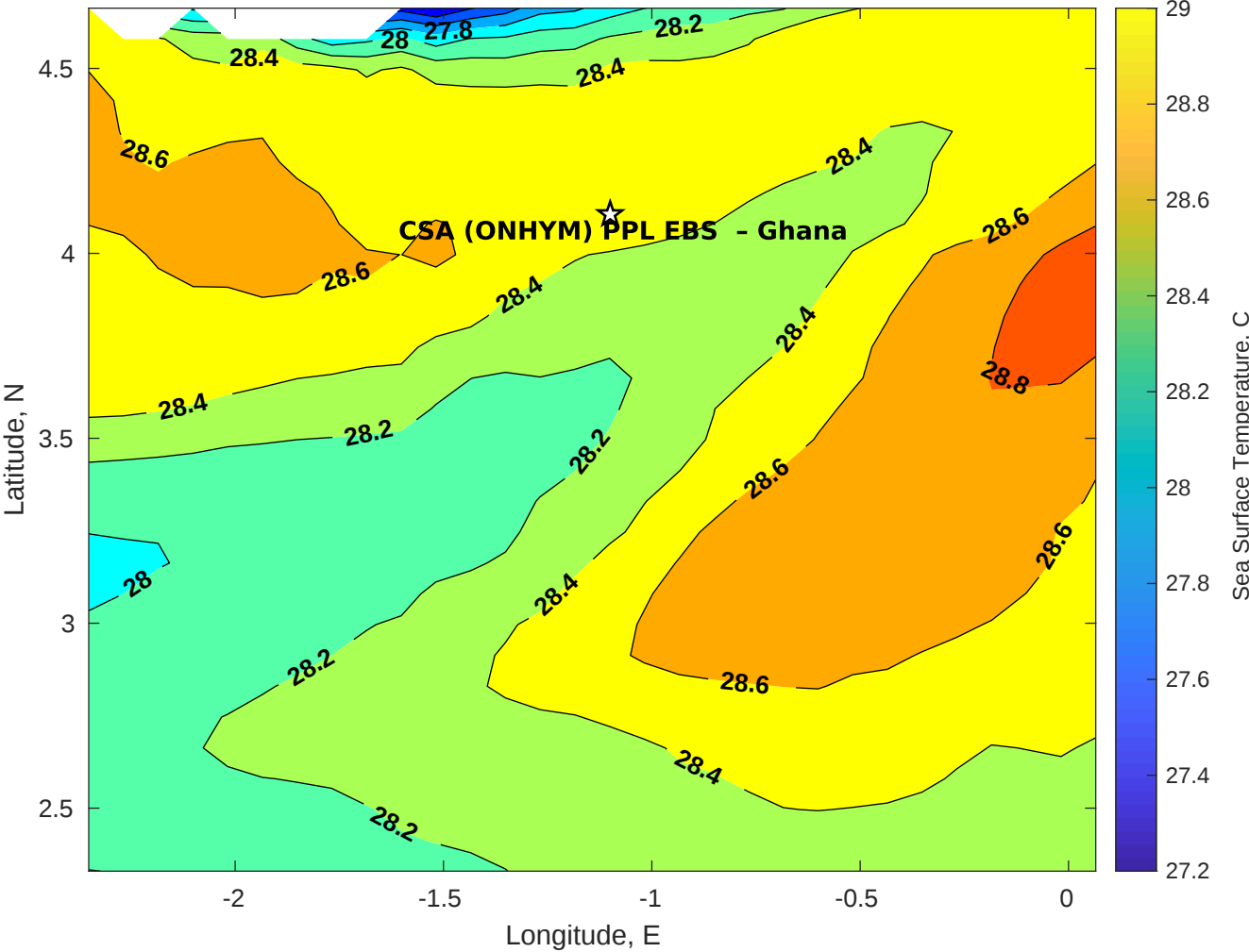
SST for CSA (ONHYM) PPL EBS - Ghana at 02-Dec-2025 00:00:00
