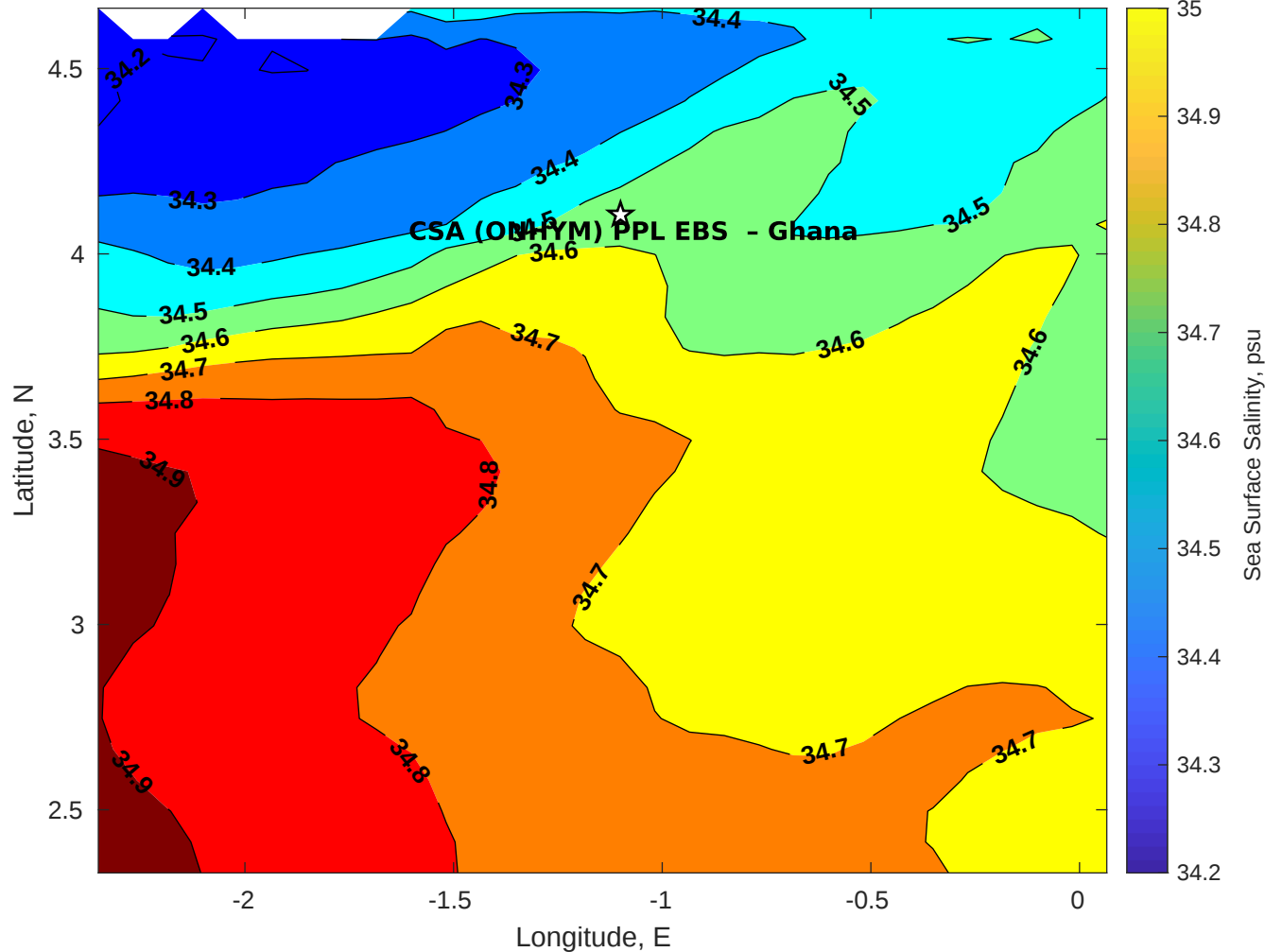
Surface Salinity for CSA (ONHYM) PPL EBS - Ghana at 02-Dec-2025 00:00:00
