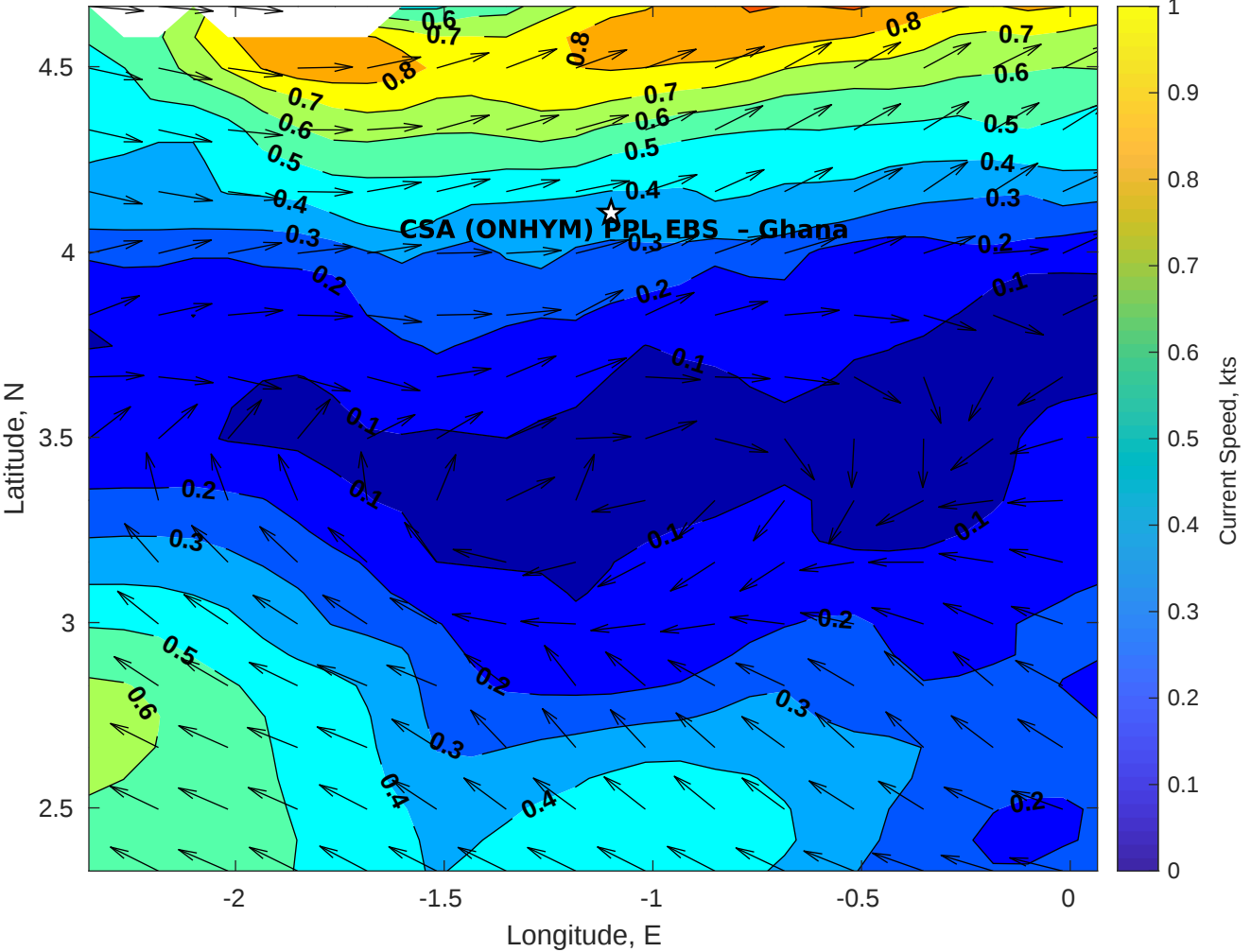
Surface Currents for CSA (ONHYM) PPL EBS - Ghana at 02-Dec-2025 00:00:00
