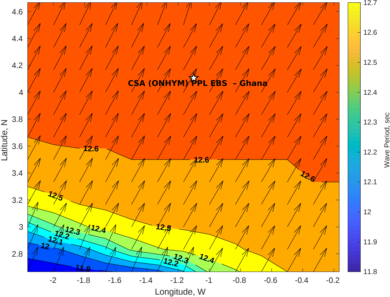
GFS Wave Period (sec) for CSA (ONHYM) PPL EBS - Ghana at 03-Dec-2025 09:00:00
