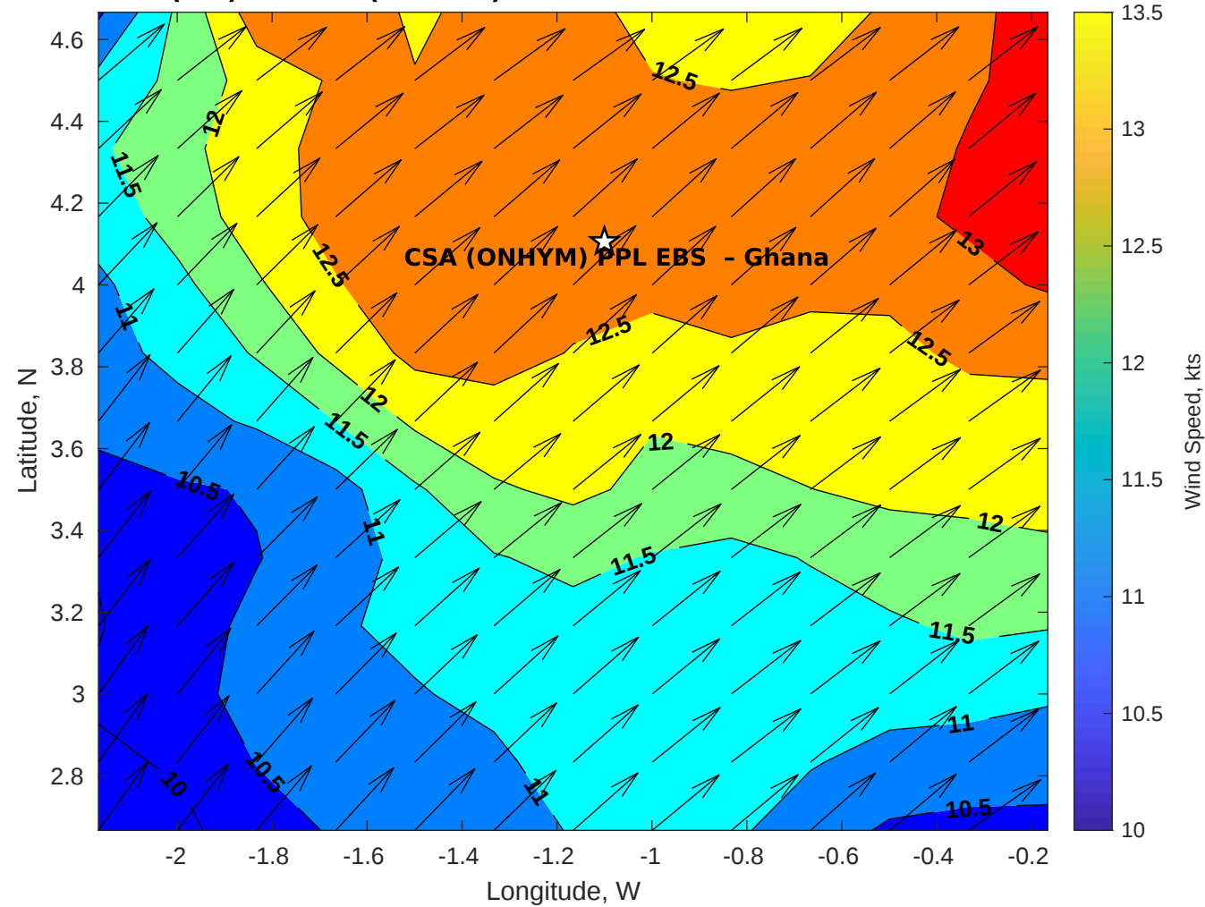
GFS Winds (kts) for CSA (ONHYM) PPL EBS - Ghana at 03-Dec-2025 09:00:00
