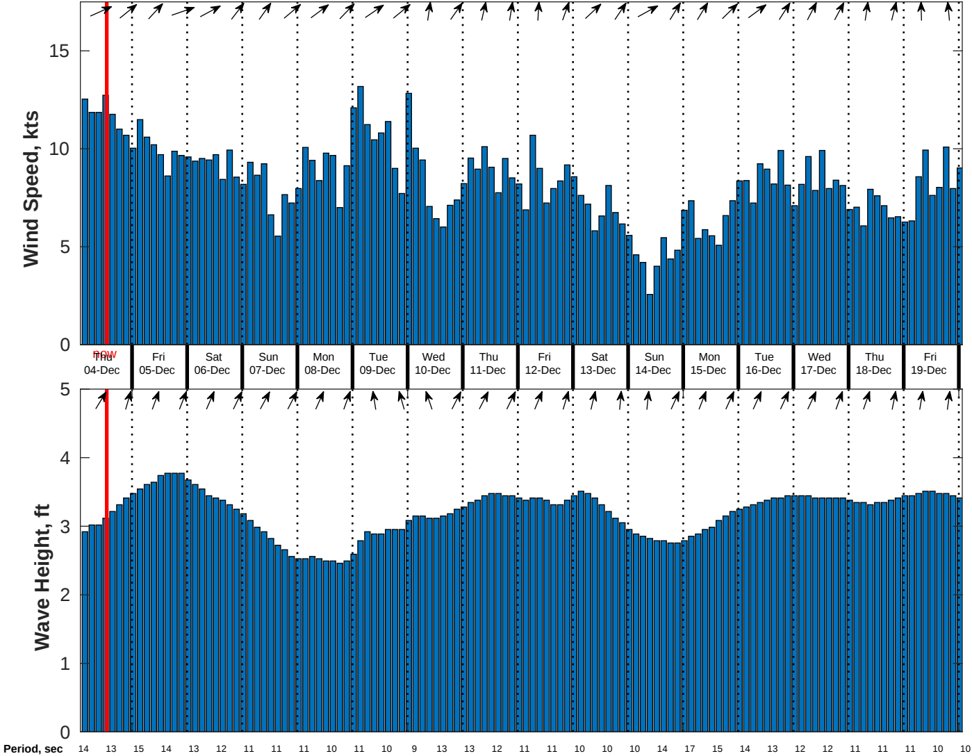
Wind & Wave Forecast for CSA (ONHYM) PPL EBS - Ghana from 03-Dec-2025 02:00:00 to 19-Dec-2025 02:00:00
