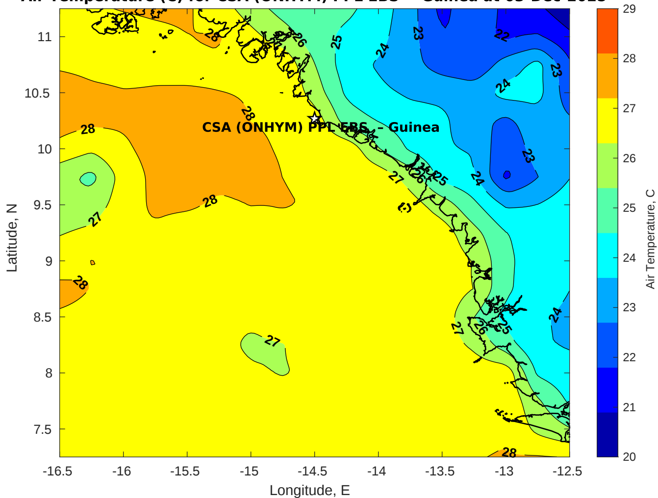
Air Temperature (C) for CSA (ONHYM) PPL EBS - Guinea at 03-Dec-2025
