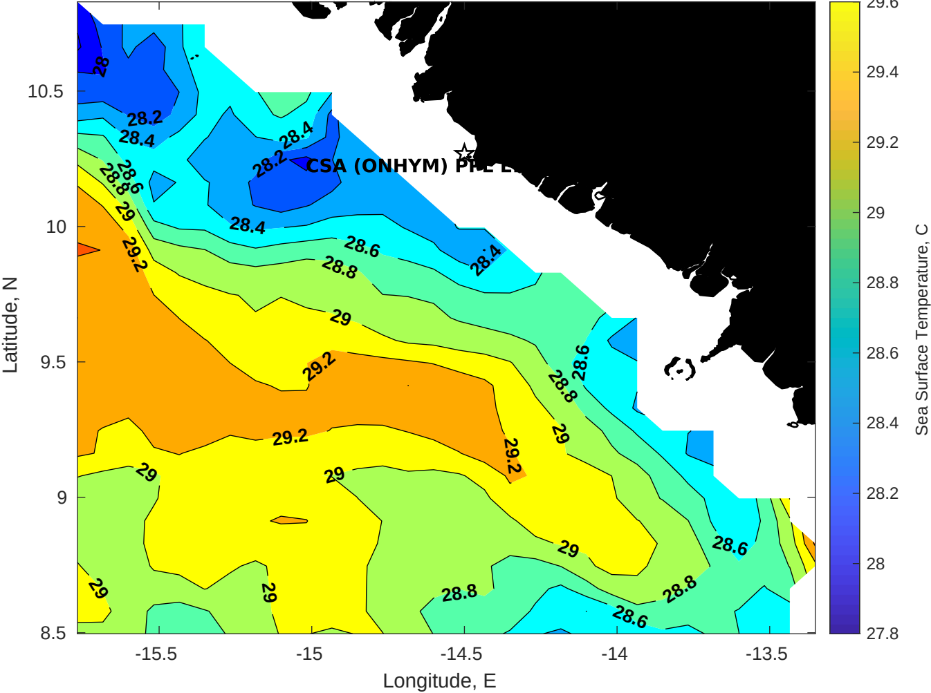
SST for CSA (ONHYM) PPL EBS - Guinea at 02-Dec-2025 00:00:00
