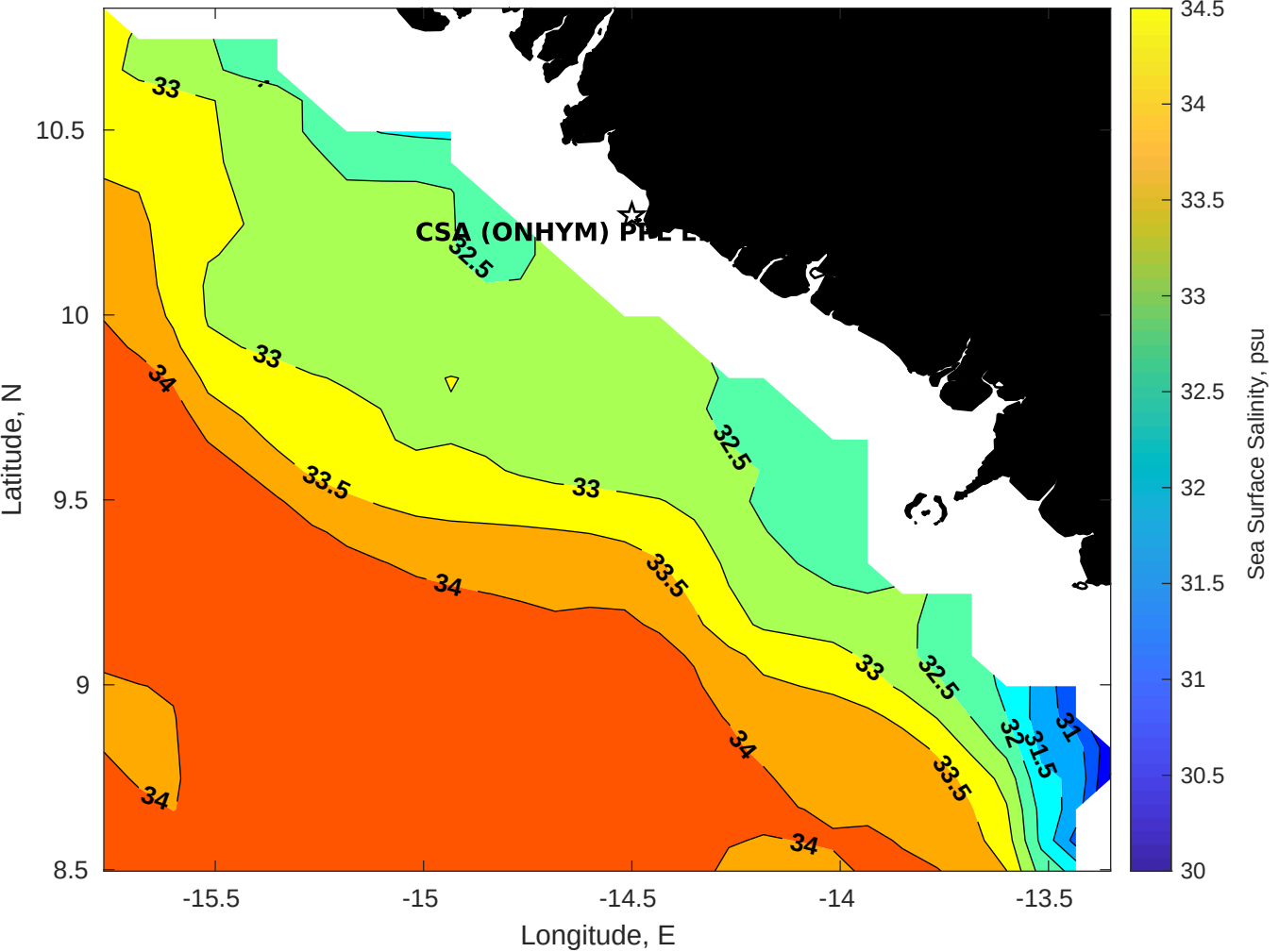
Surface Salinity for CSA (ONHYM) PPL EBS - Guinea at 02-Dec-2025 00:00:00
