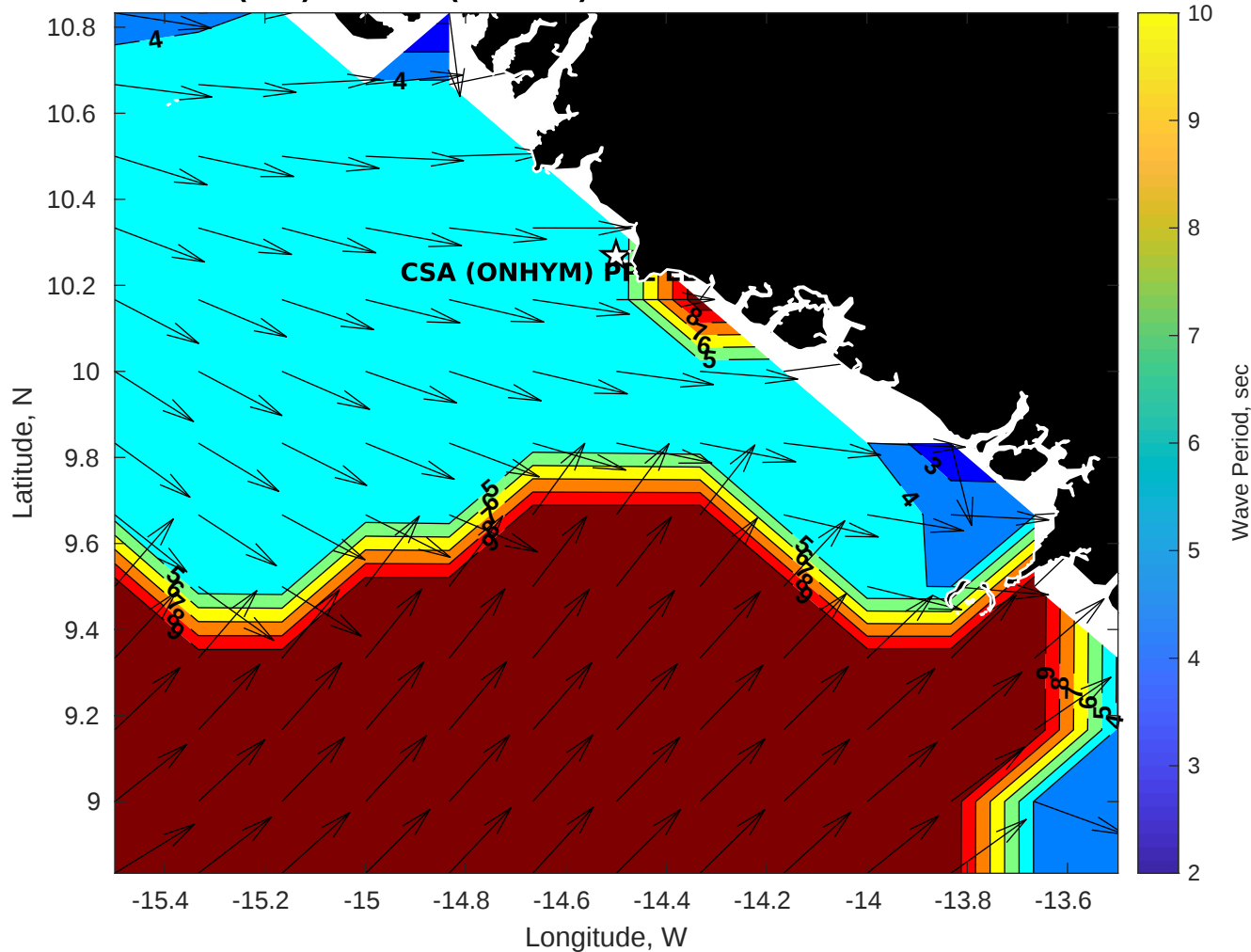
GFS Wave Period (sec) for CSA (ONHYM) PPL EBS - Guinea at 03-Dec-2025 09:00:00
