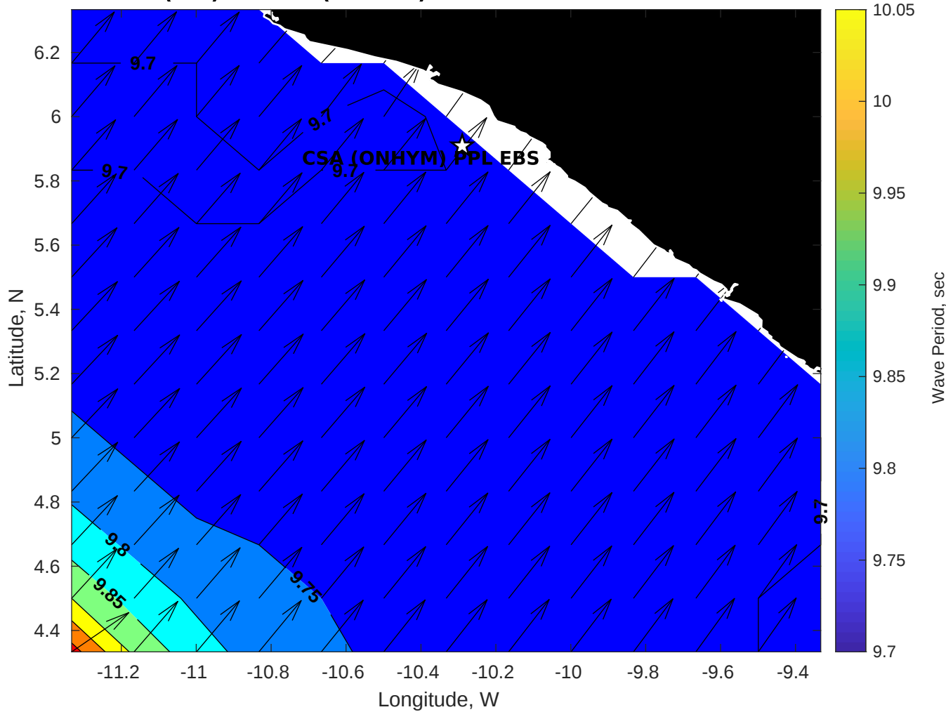
GFS Wave Period (sec) for CSA (ONHYM) PPL EBS - Liberia at 03-Dec-2025 09:00:00
