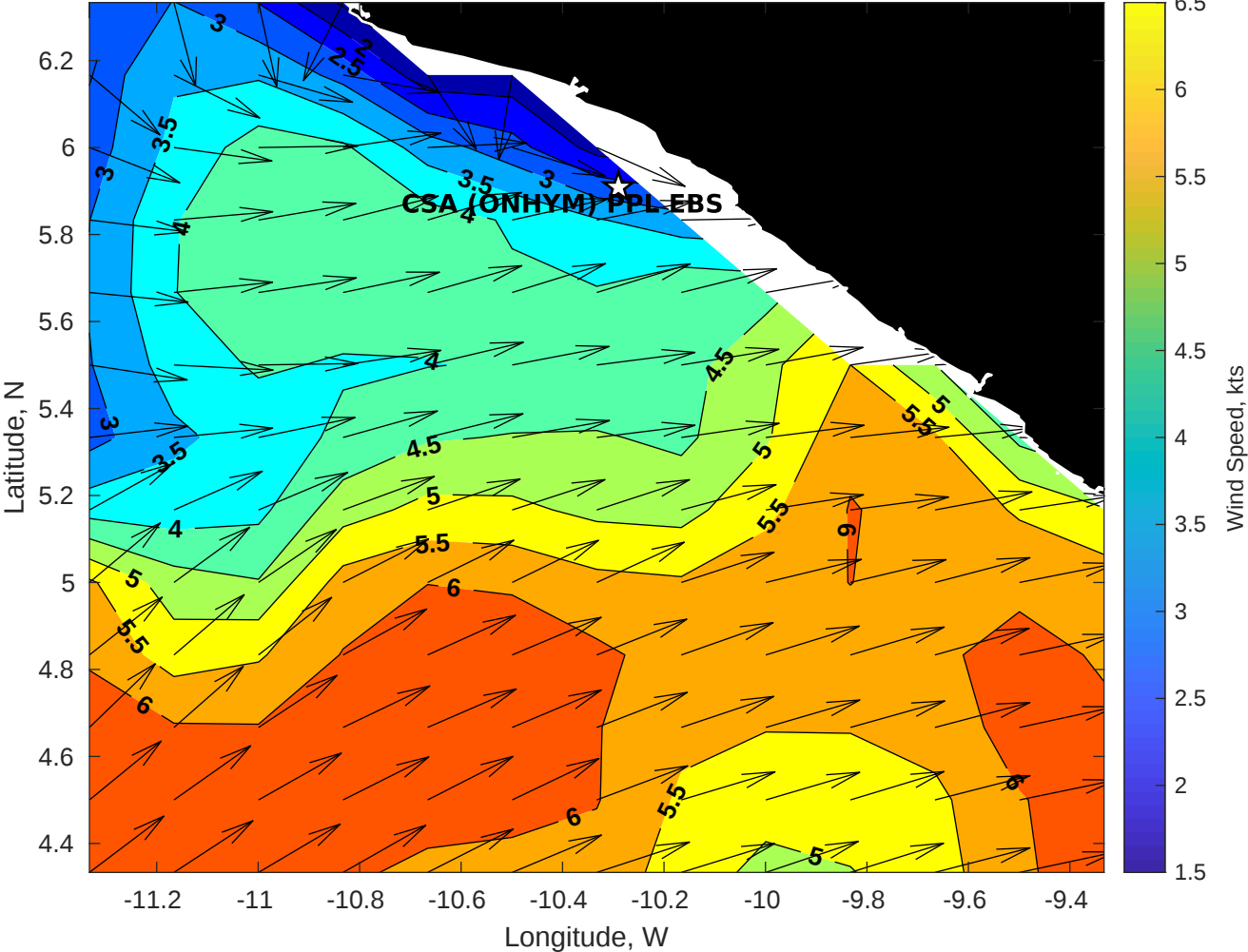
GFS Winds (kts) for CSA (ONHYM) PPL EBS - Liberia at 03-Dec-2025 09:00:00
