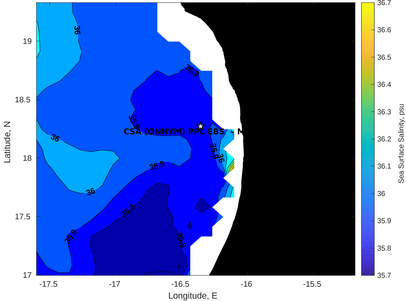
Surface Salinity for CSA (ONHYM) PPL EBS - Mauritania at 02-Dec-2025 00:00:00
