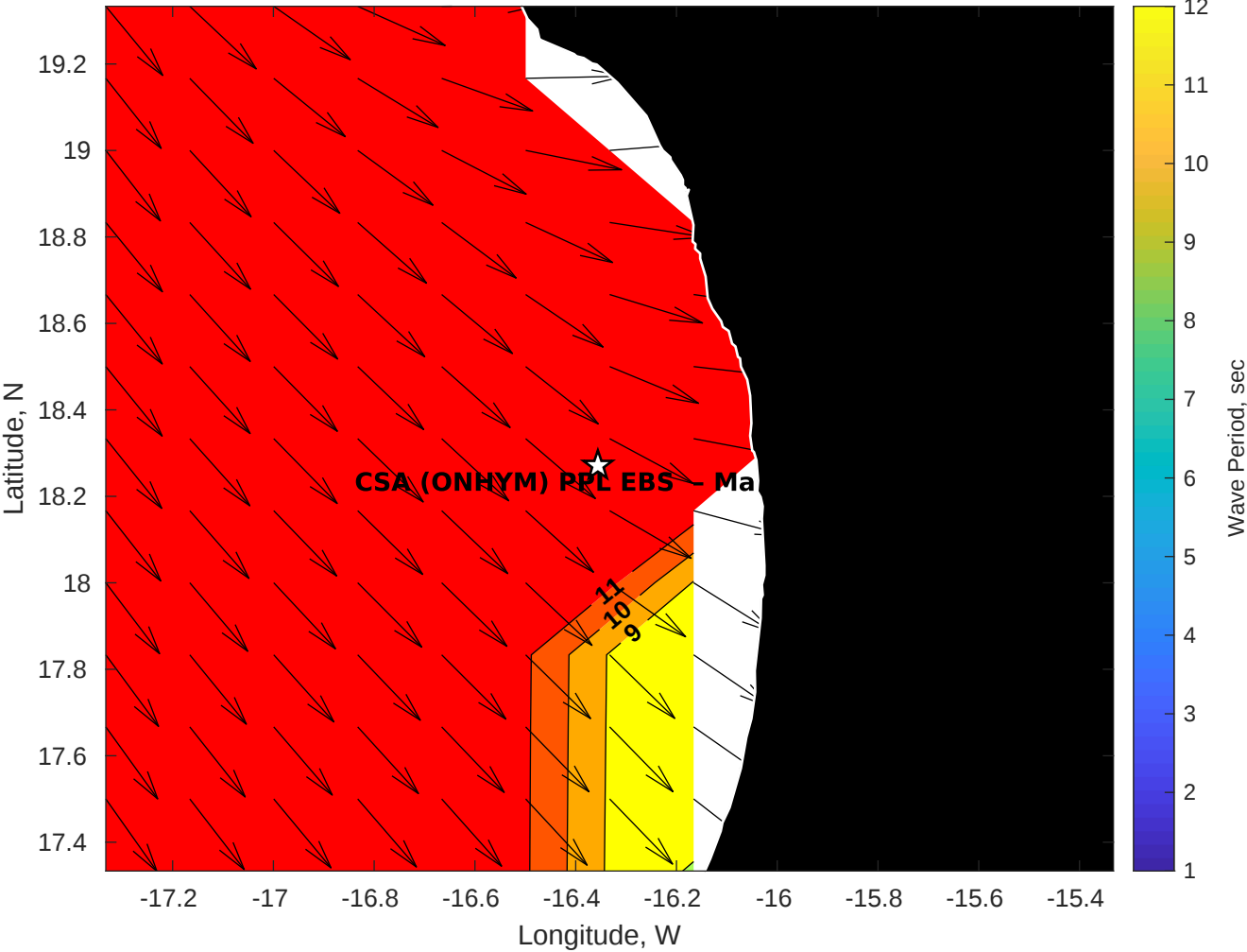
GFS Wave Period (sec) for CSA (ONHYM) PPL EBS - Mauritania at 03-Dec-2025 09:00:00
