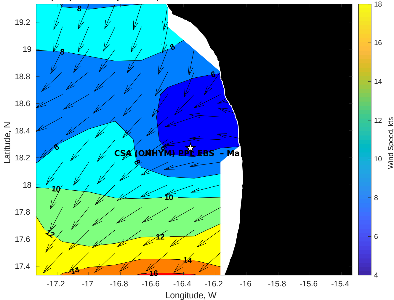
GFS Winds (kts) for CSA (ONHYM) PPL EBS - Mauritania at 03-Dec-2025 09:00:00
