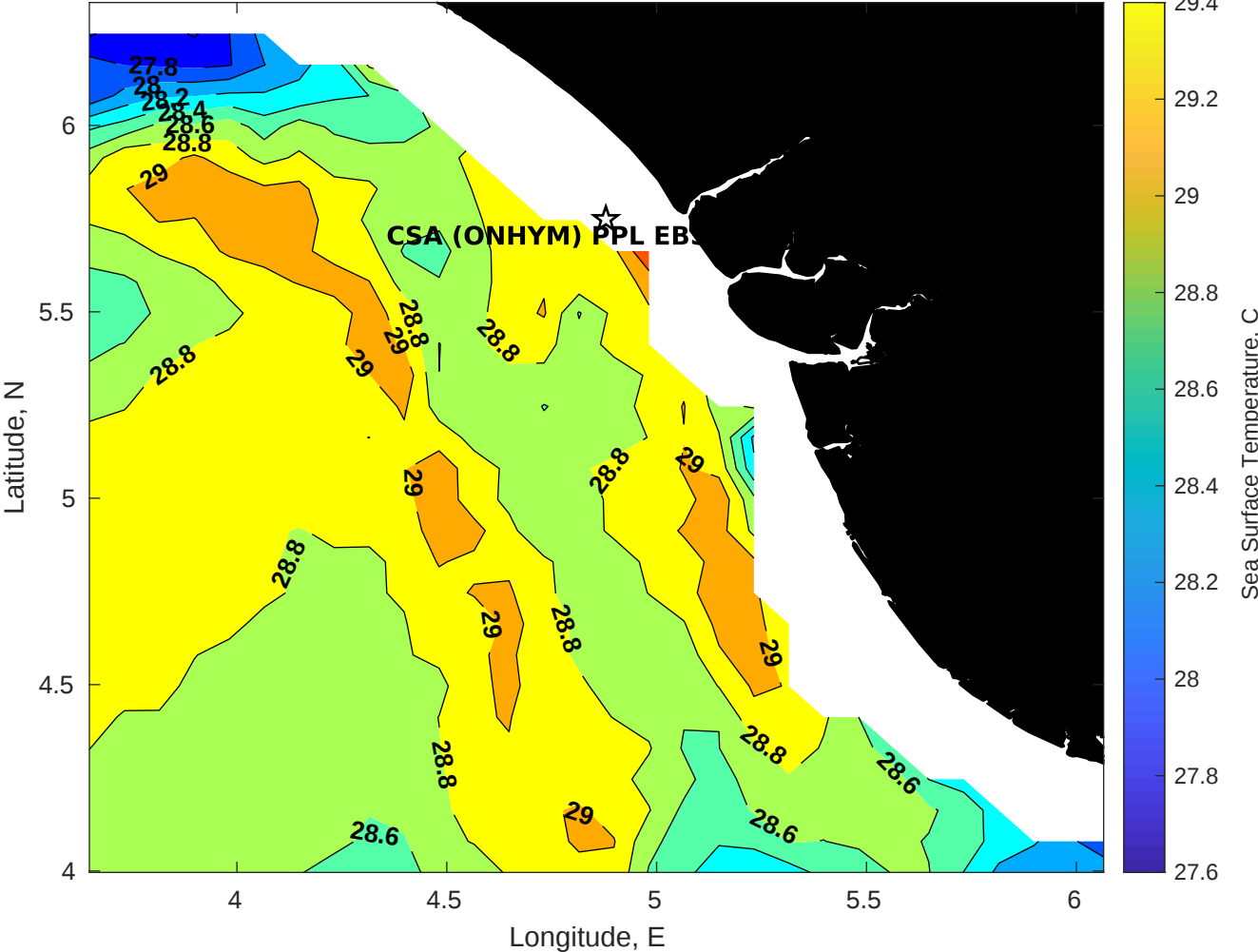
SST for CSA (ONHYM) PPL EBS - Nigeria at 02-Dec-2025 00:00:00
