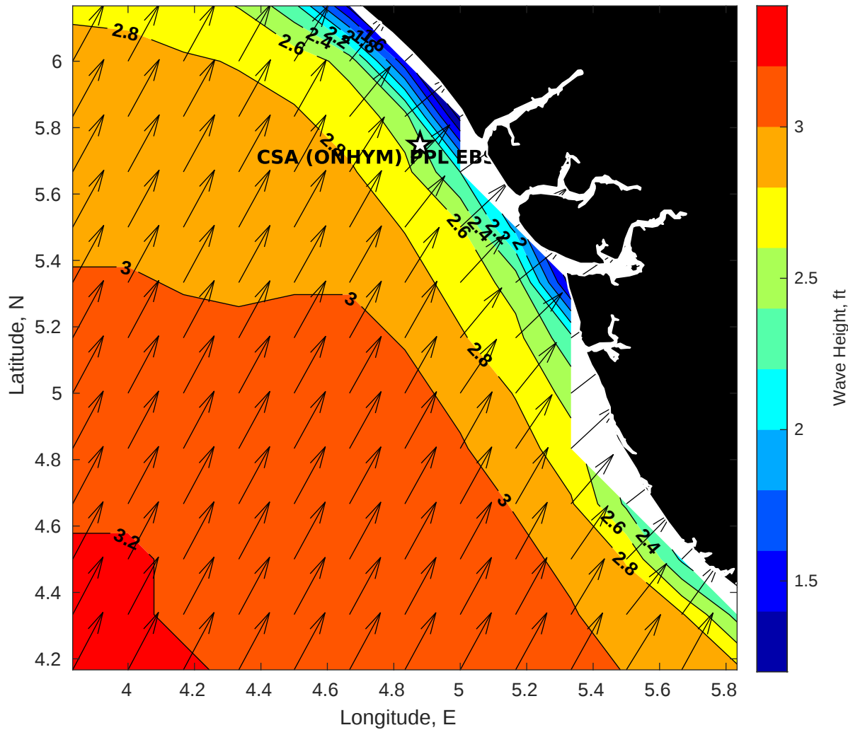
GFS Wave Height (ft) for CSA (ONHYM) PPL EBS - Nigeria at 03-Dec-2025 09:00:00
