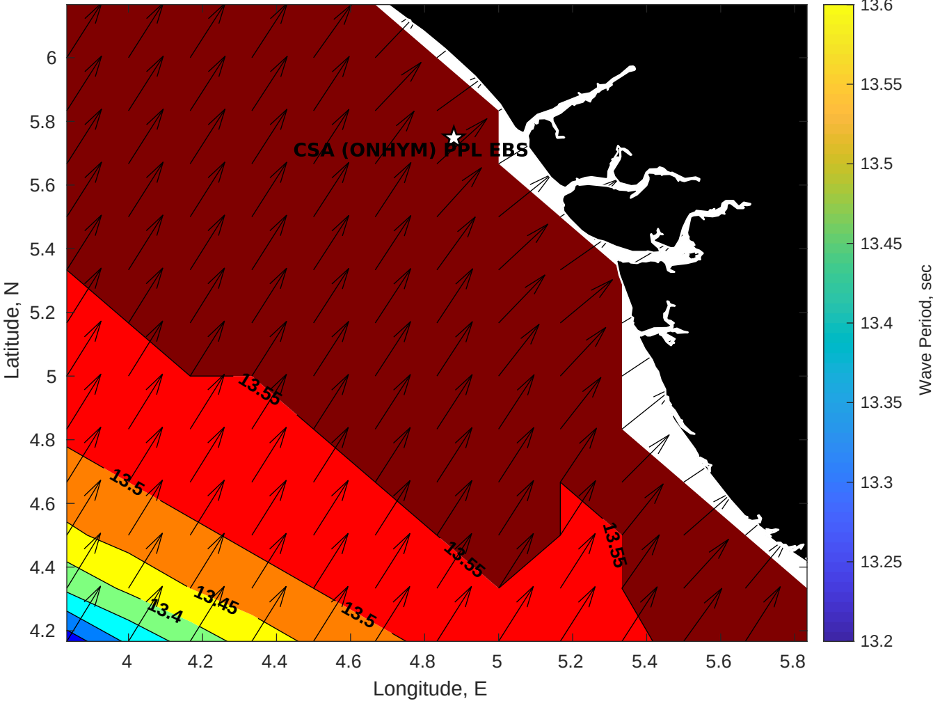
GFS Wave Period (sec) for CSA (ONHYM) PPL EBS - Nigeria at 03-Dec-2025 09:00:00
