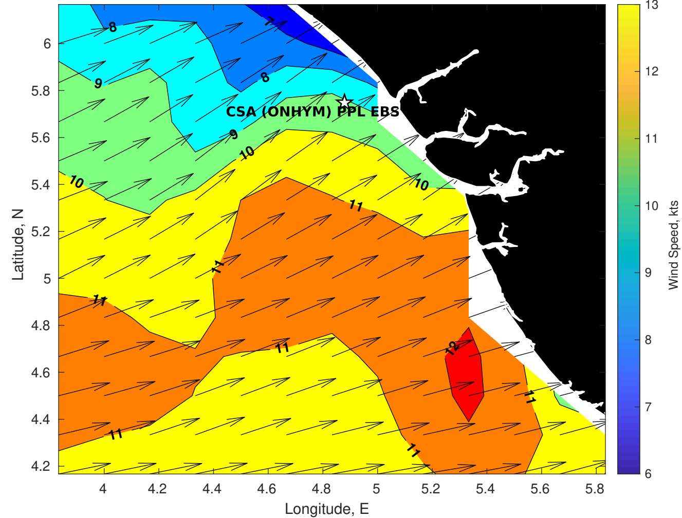
GFS Winds (kts) for CSA (ONHYM) PPL EBS - Nigeria at 03-Dec-2025 09:00:00
