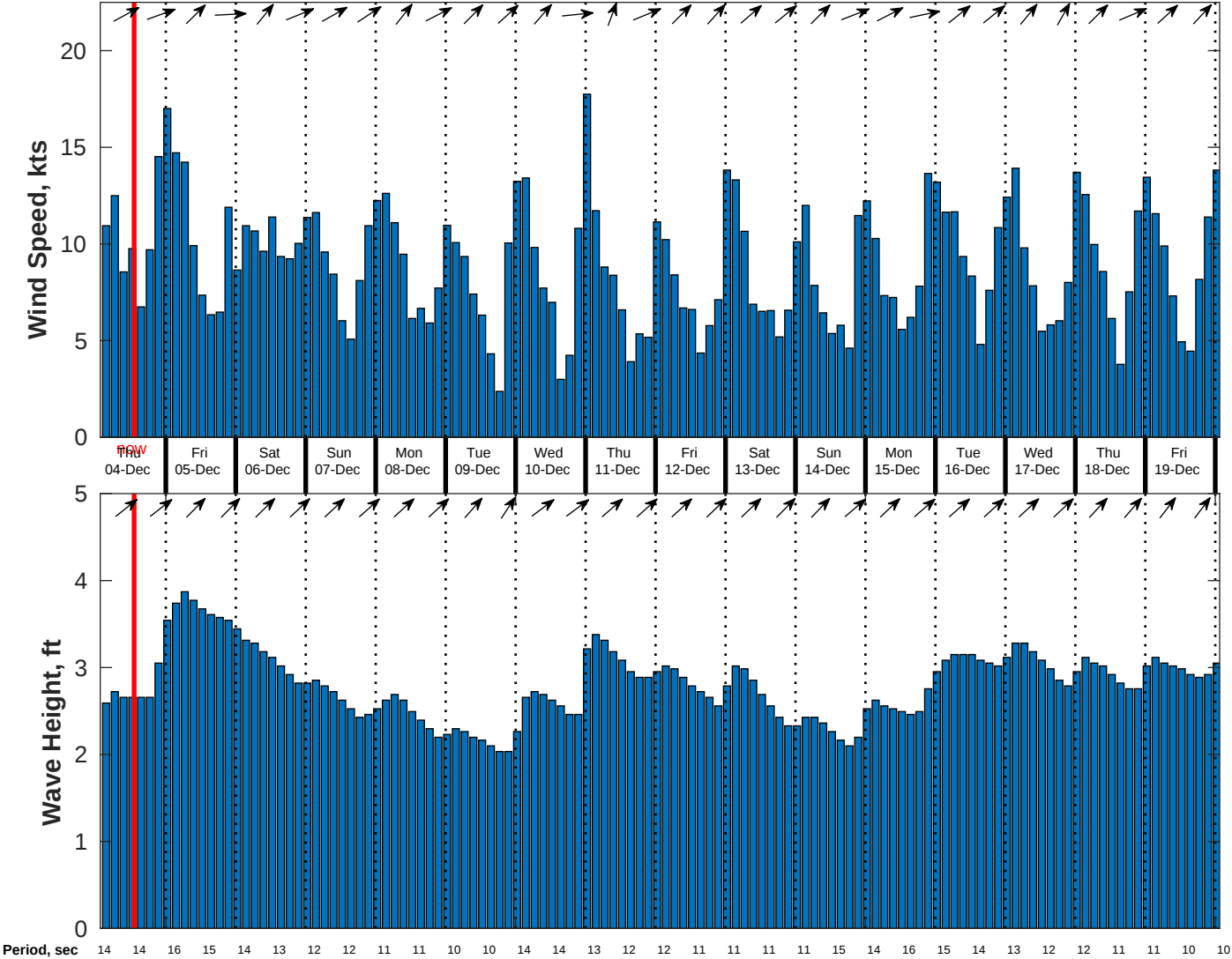
Wind & Wave Forecast for CSA (ONHYM) PPL EBS - Nigeria from 03-Dec-2025 02:00:00 to 19-Dec-2025 02:00:00
