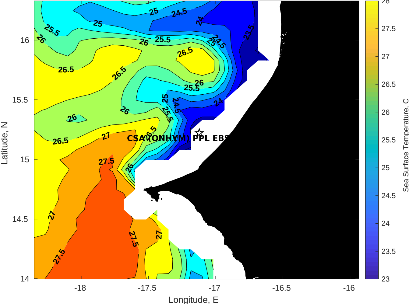
SST for CSA (ONHYM) PPL EBS - Senegal at 02-Dec-2025 00:00:00
