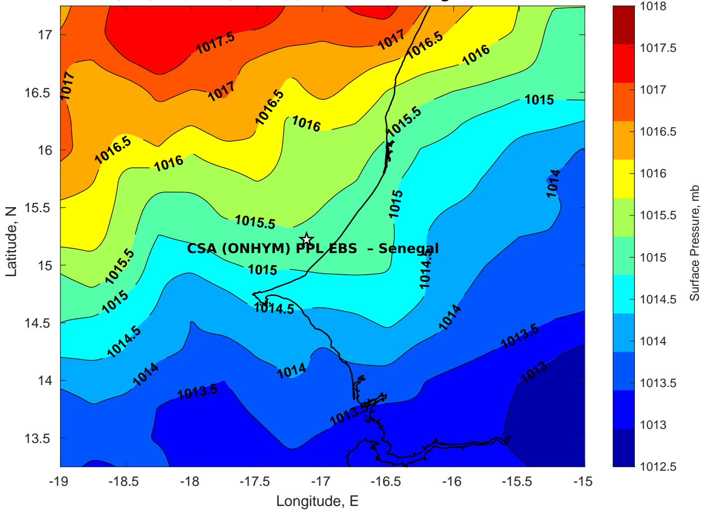
Surface Pressure (mb) for CSA (ONHYM) PPL EBS - Senegal at 03-Dec-2025 00:00:00
