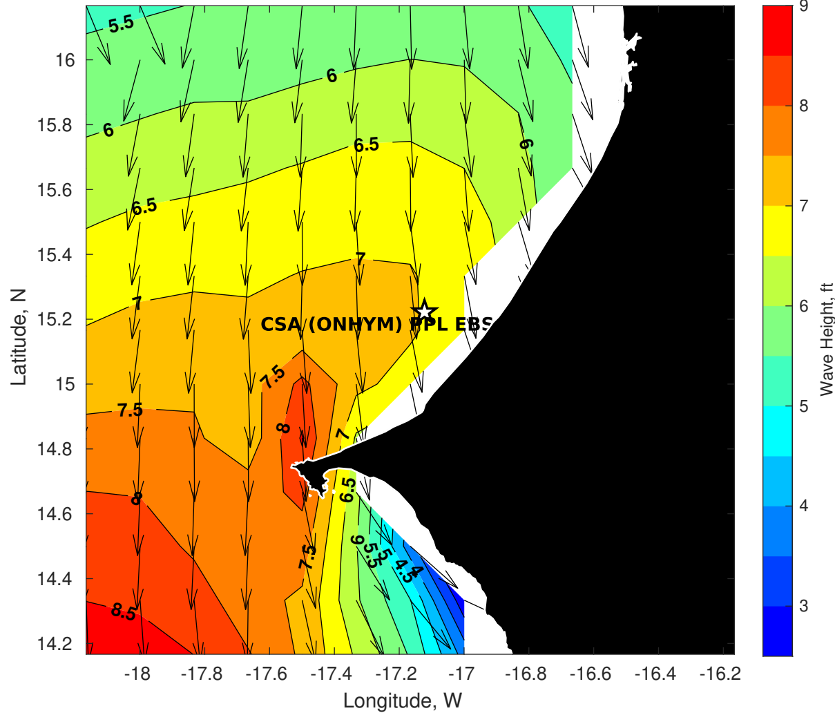
GFS Wave Height (ft) for CSA (ONHYM) PPL EBS - Senegal at 03-Dec-2025 09:00:00
