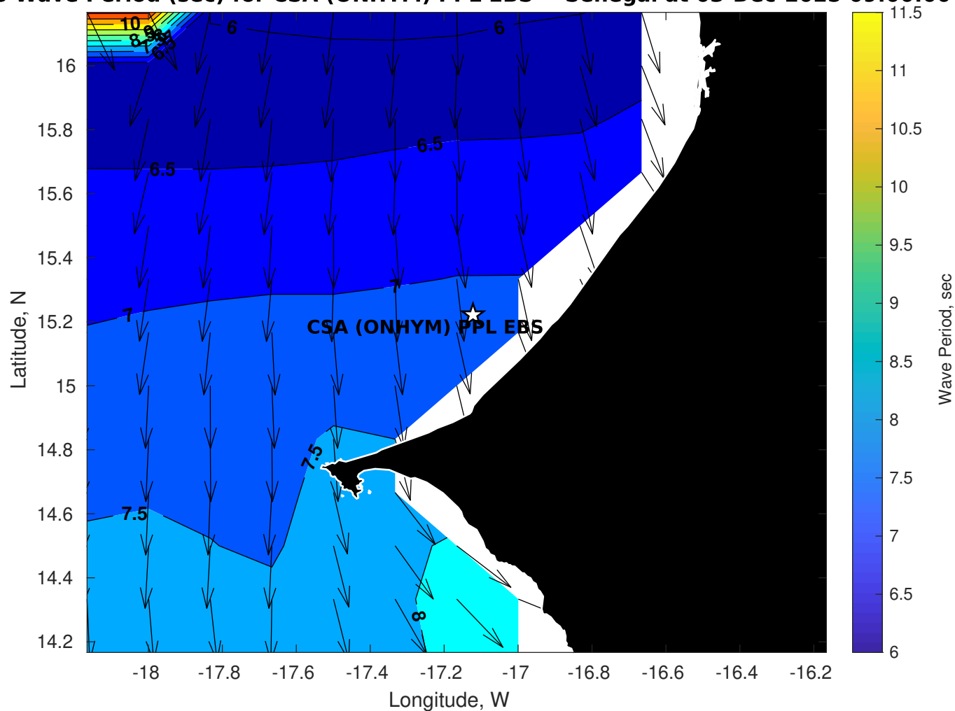
GFS Wave Period (sec) for CSA (ONHYM) PPL EBS - Senegal at 03-Dec-2025 09:00:00
