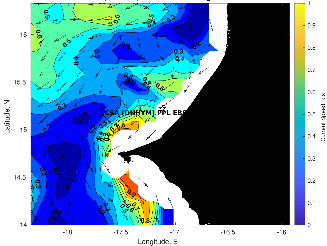
Surface Currents for CSA (ONHYM) PPL EBS - Senegal at 02-Dec-2025 00:00:00
