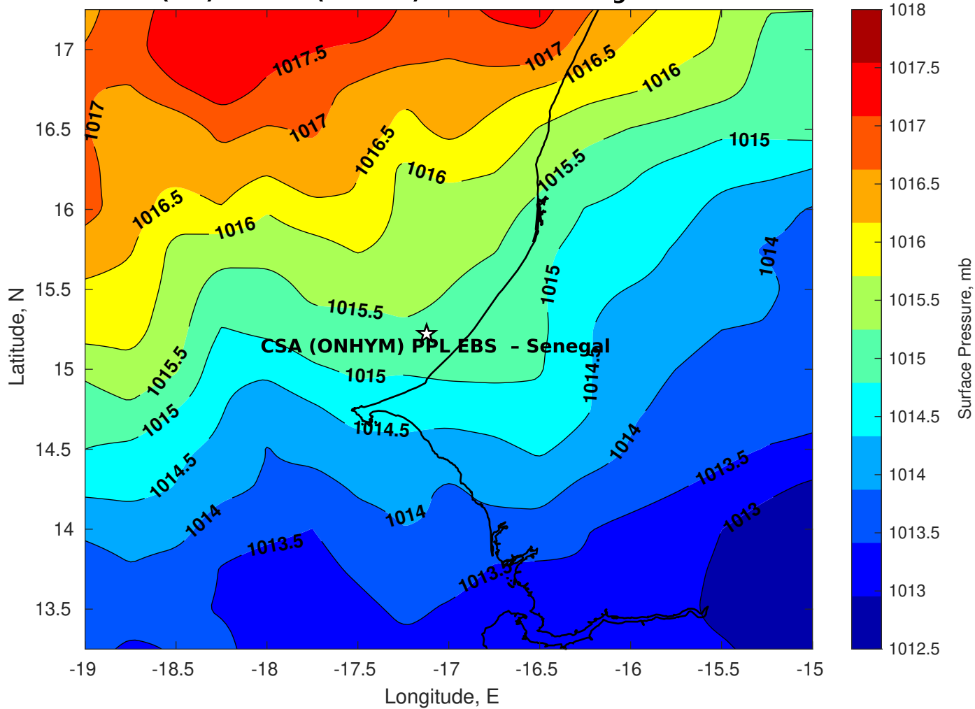
Surface Pressure (mb) for CSA (ONHYM) PPL EBS - Senegal at 03-Dec-2025 00:00:00
