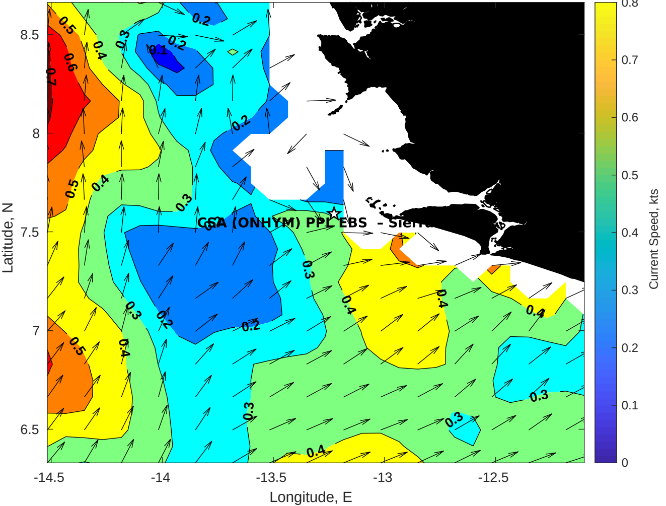
Surface Currents for CSA (ONHYM) PPL EBS - Sierra Leone at 02-Dec-2025 00:00:00
