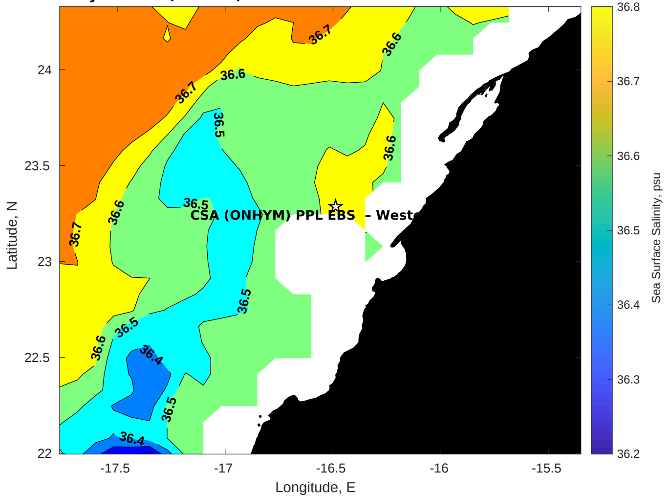
Surface Salinity for CSA (ONHYM) PPL EBS - Western Sahara at 02-Dec-2025 00:00:00
