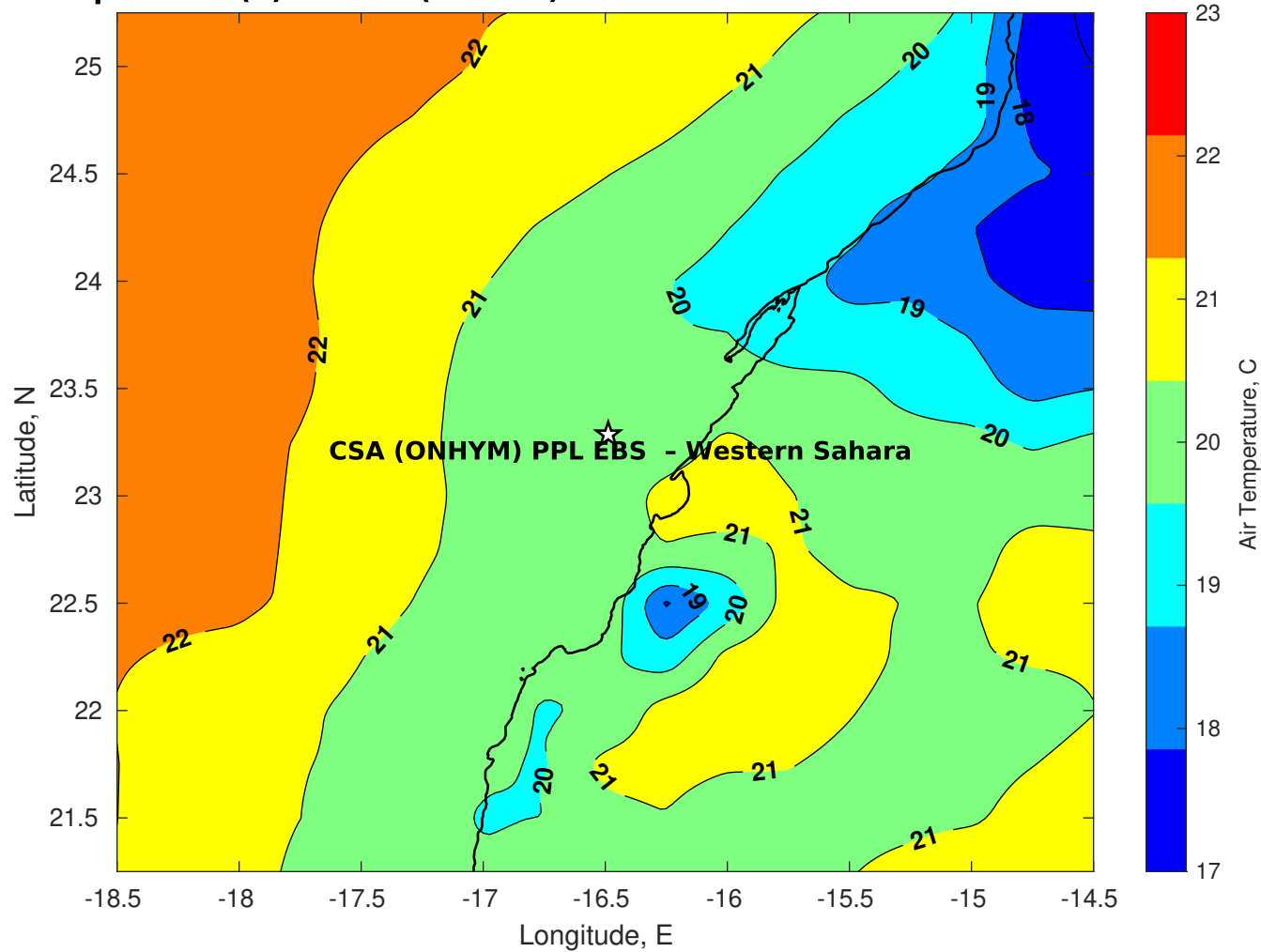
Air Temperature (C) for CSA (ONHYM) PPL EBS - Western Sahara at 03-Dec-2025
