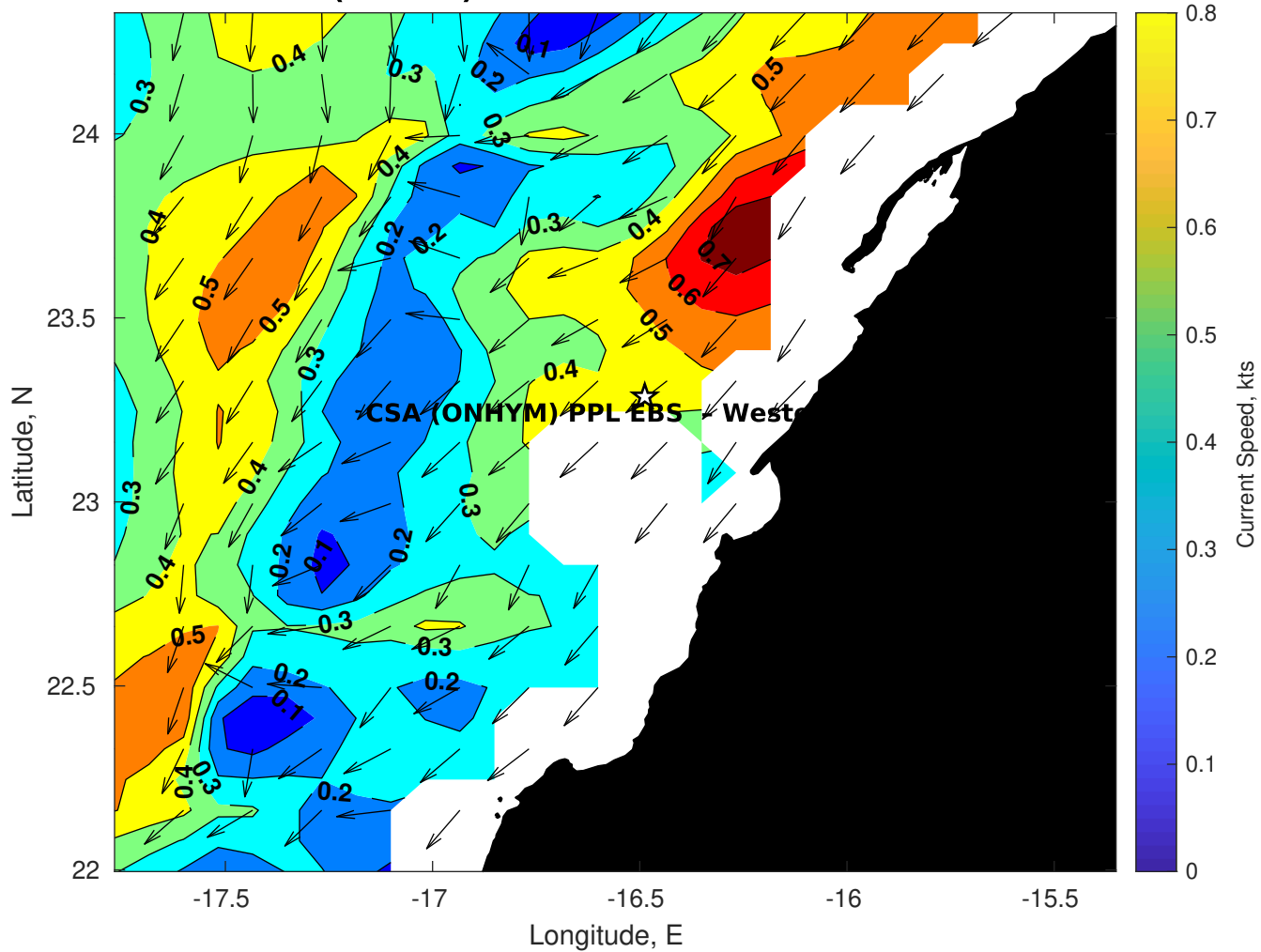
Surface Currents for CSA (ONHYM) PPL EBS - Western Sahara at 02-Dec-2025 00:00:00
