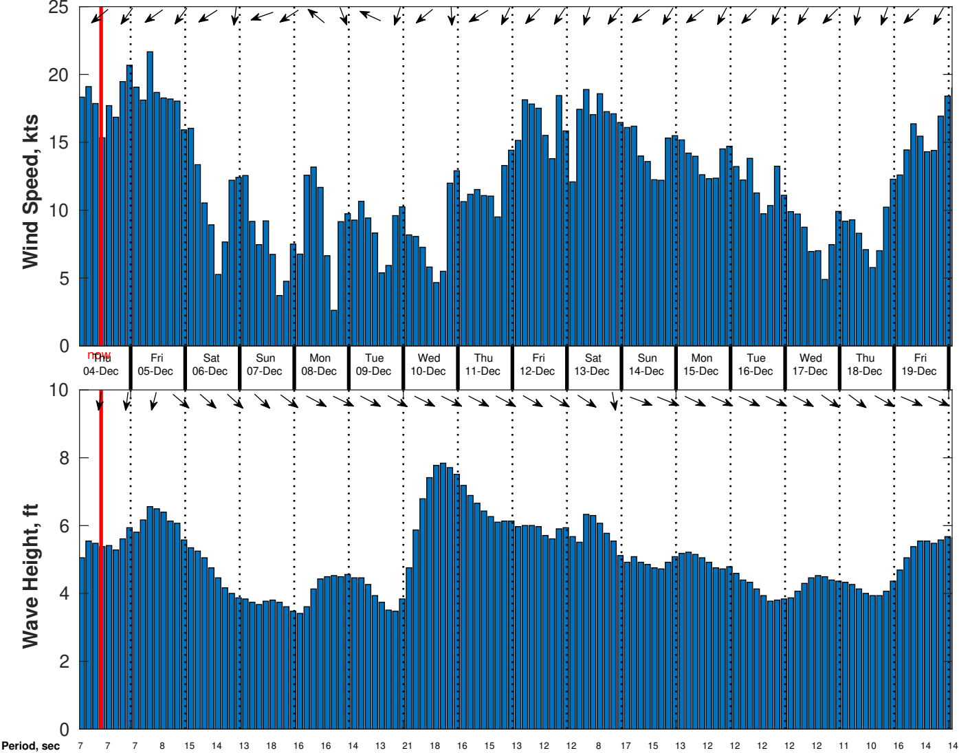
Wind & Wave Forecast for CSA (ONHYM) PPL EBS - Western Sahara from 03-Dec-2025 01:00:00 to 19-Dec-2025 01:00:00
