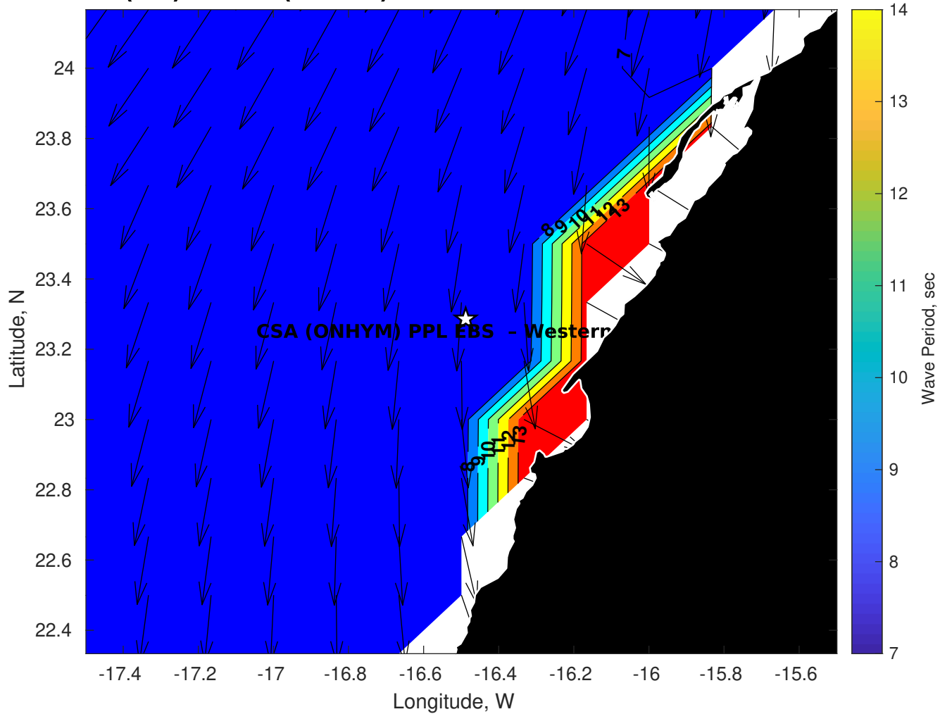
GFS Wave Period (sec) for CSA (ONHYM) PPL EBS - Western Sahara at 03-Dec-2025 09:00:00
