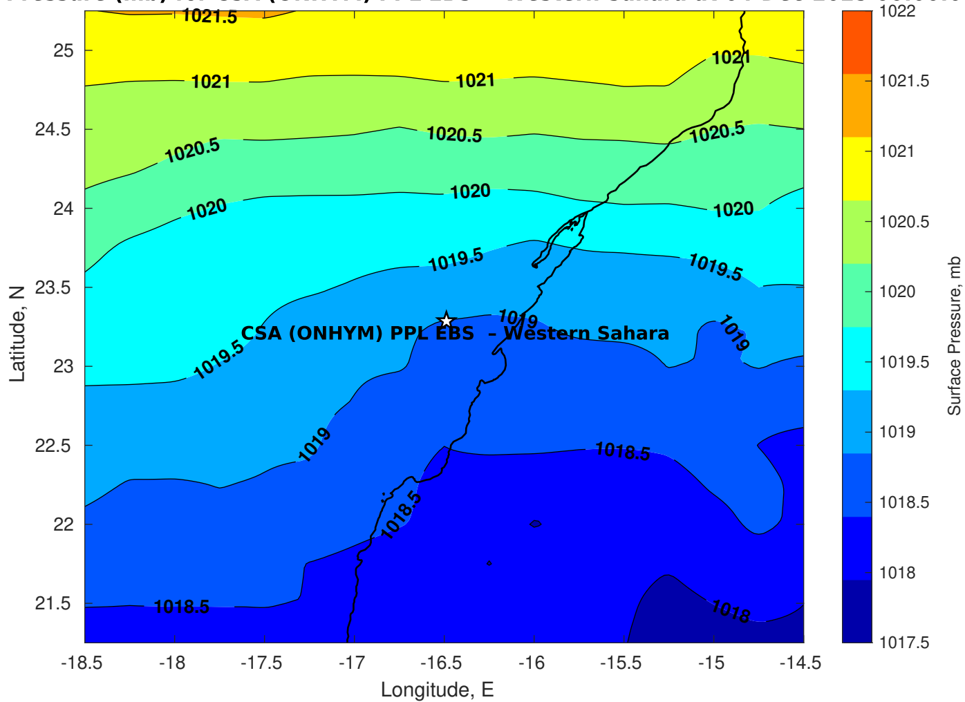
Surface Pressure (mb) for CSA (ONHYM) PPL EBS - Western Sahara at 04-Dec-2025 00:00:00
