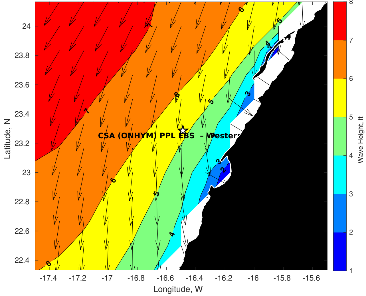
GFS Wave Height (ft) for CSA (ONHYM) PPL EBS - Western Sahara at 03-Dec-2025 09:00:00
