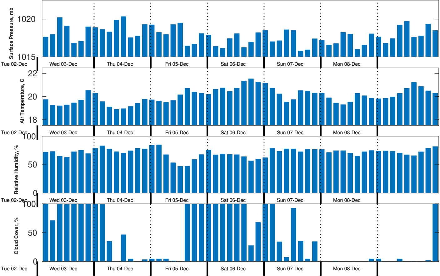
Met Forecast for CSA (ONHYM) PPL EBS - Western Sahara from 03-Dec-2025 00:00:00 to 10-Dec-2025 00:00:00
