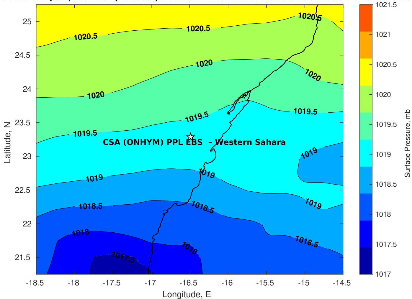
Surface Pressure (mb) for CSA (ONHYM) PPL EBS - Western Sahara at 05-Dec-2025 00:00:00
