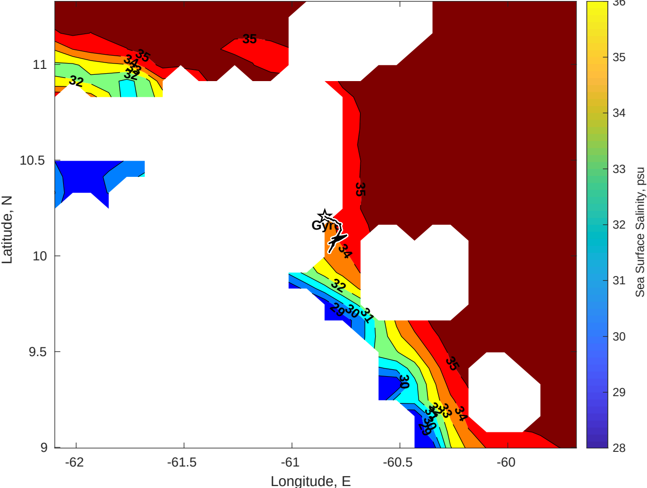
Surface Salinity for Gyre at 02-Dec-2025 00:00:00
