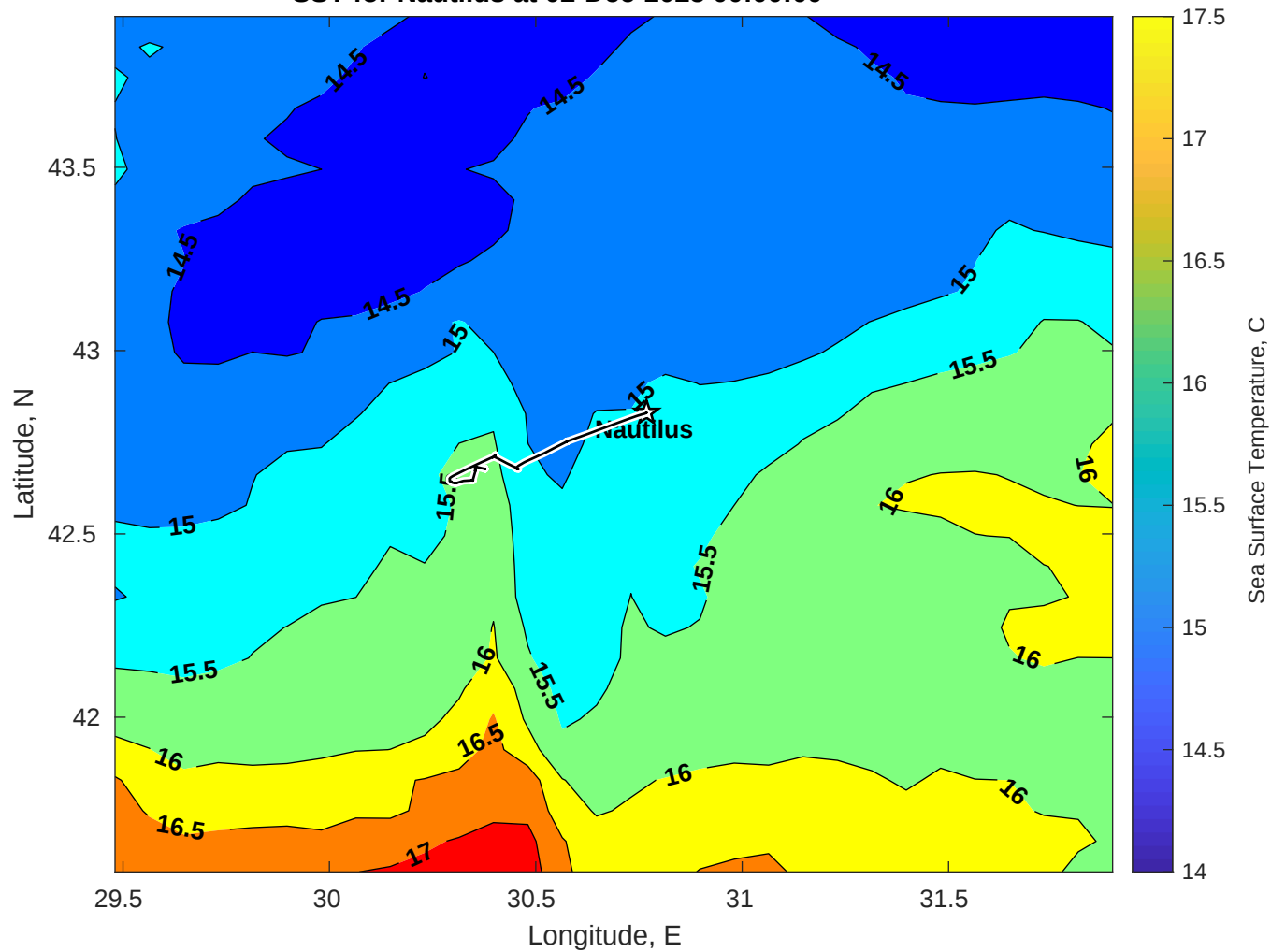
SST for Nautilus at 02-Dec-2025 00:00:00
