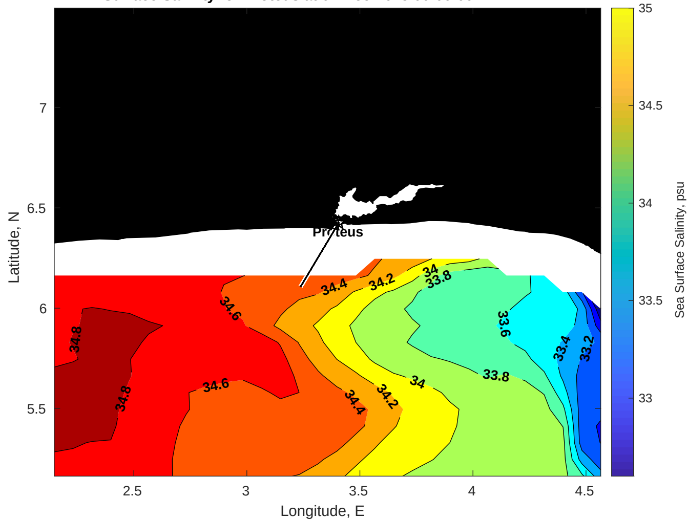
Surface Salinity for Proteus at 02-Dec-2025 00:00:00
