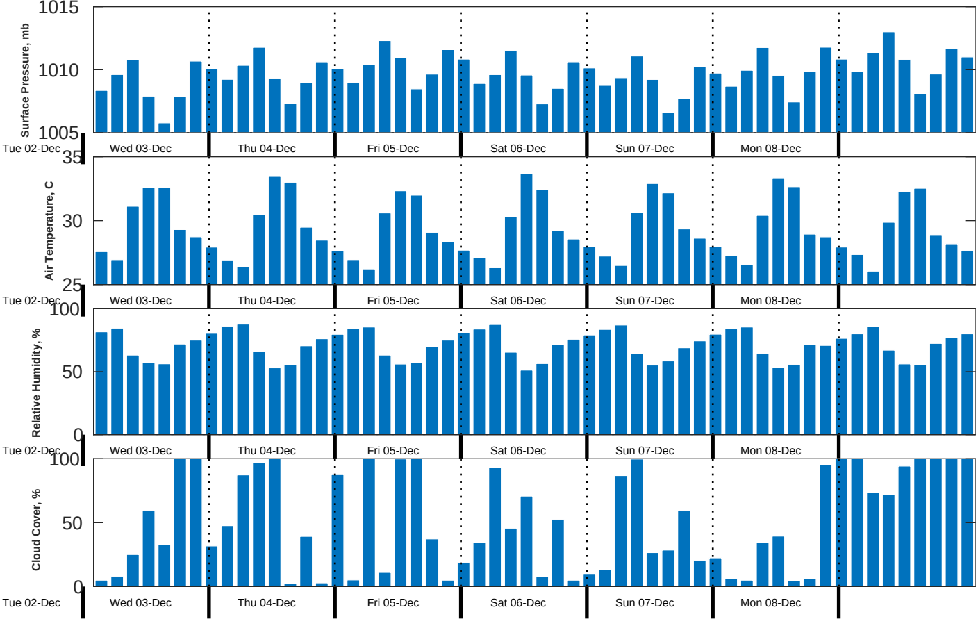
Met Forecast for Proteus from 03-Dec-2025 00:00:00 to 10-Dec-2025 00:00:00
