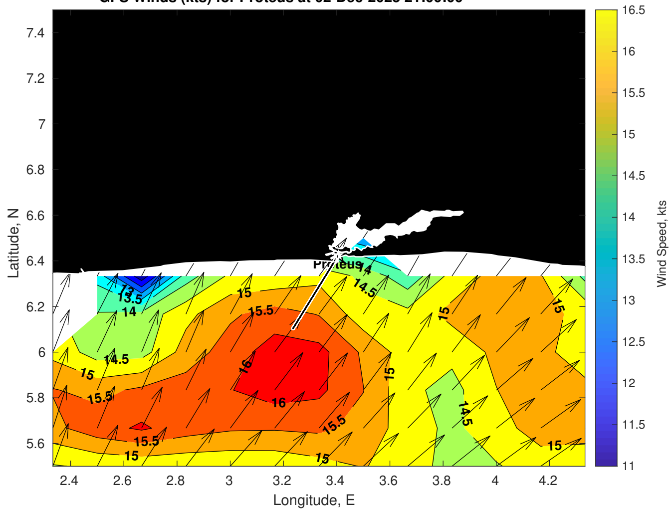
GFS Winds (kts) for Proteus at 02-Dec-2025 21:00:00
