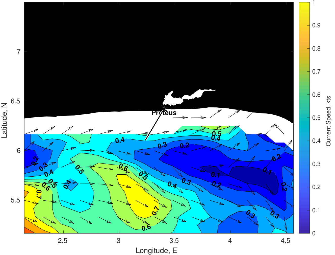
Surface Currents for Proteus at 02-Dec-2025 00:00:00
