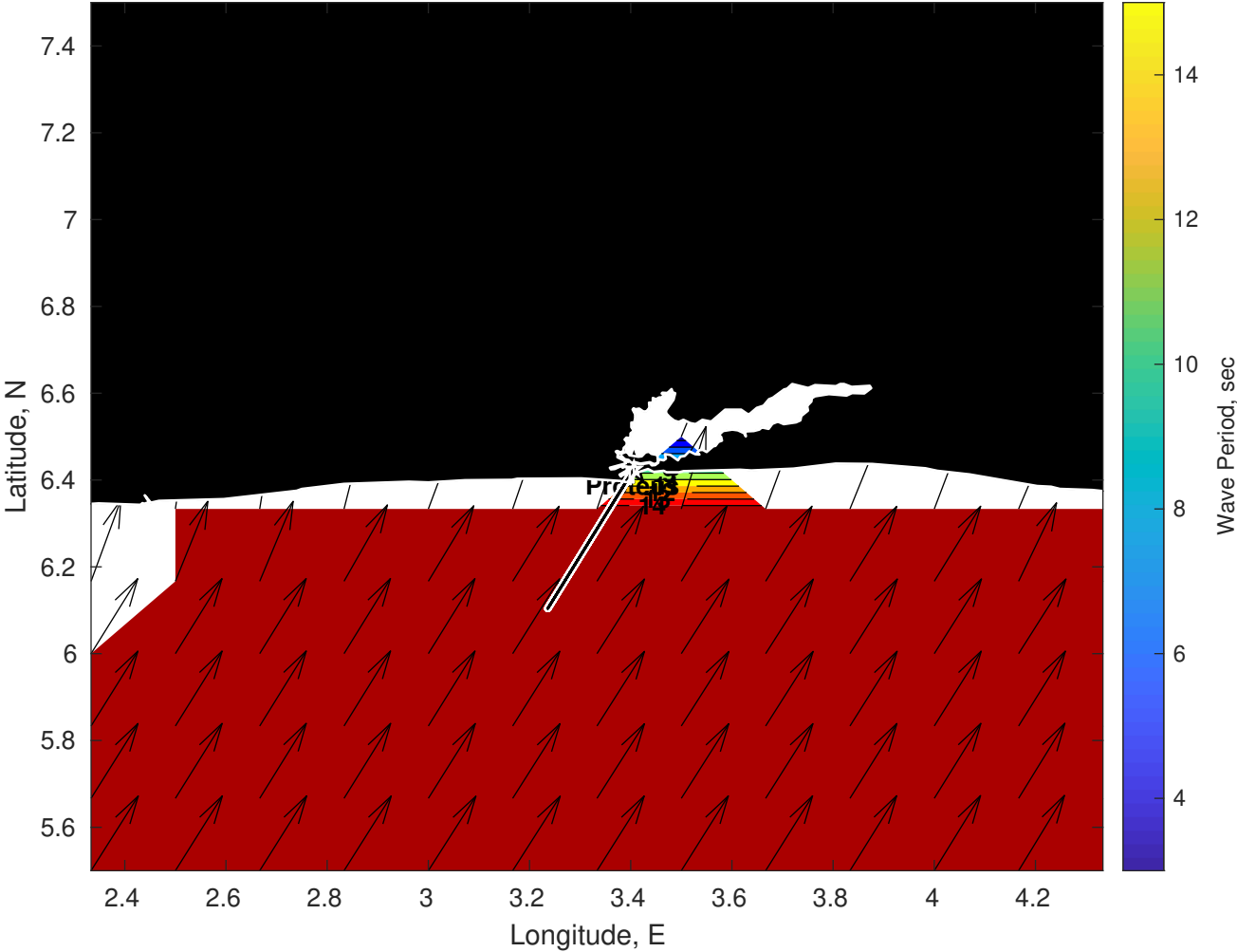
GFS Wave Period (sec) for Proteus at 02-Dec-2025 21:00:00
