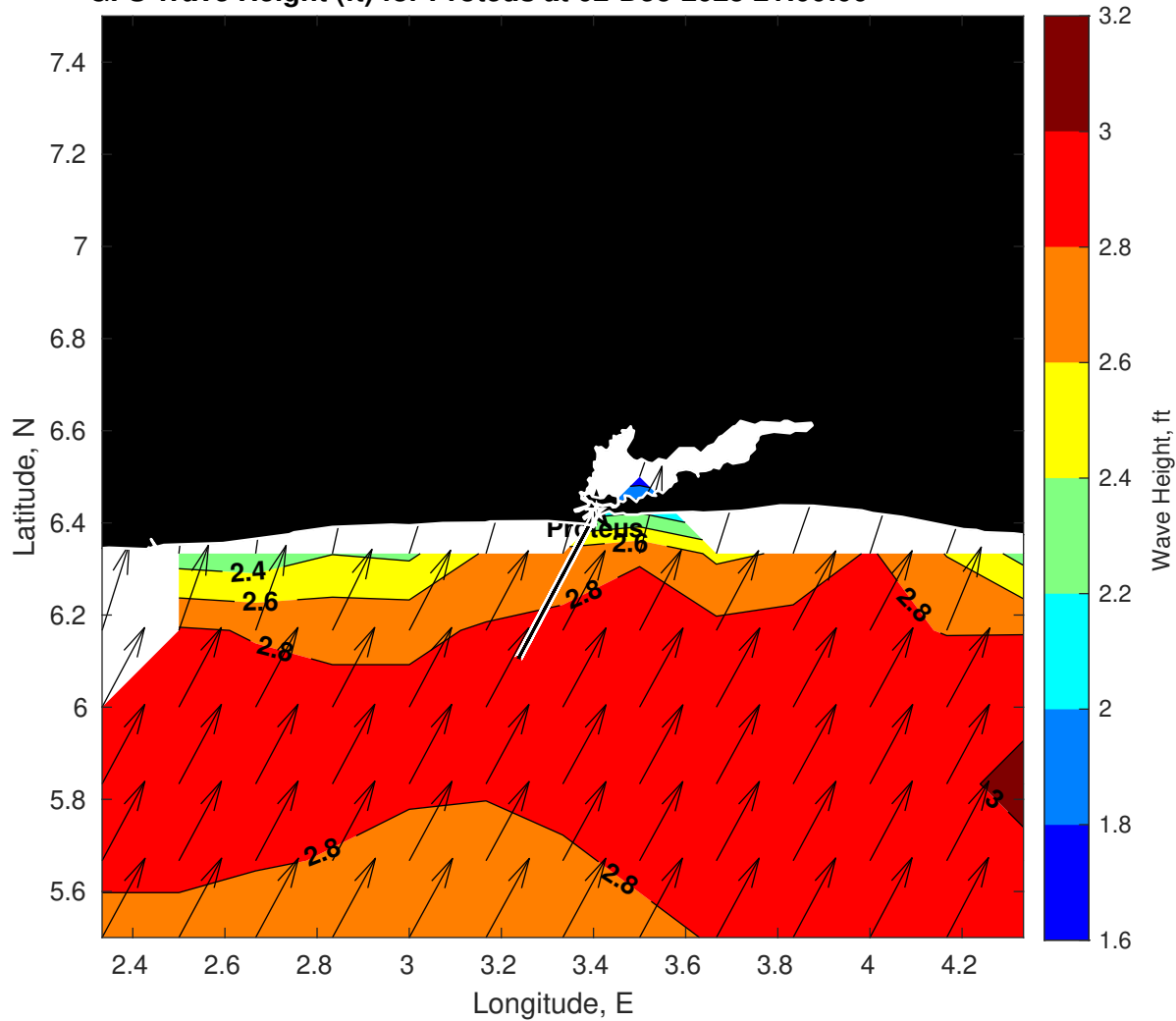
GFS Wave Height (ft) for Proteus at 02-Dec-2025 21:00:00
