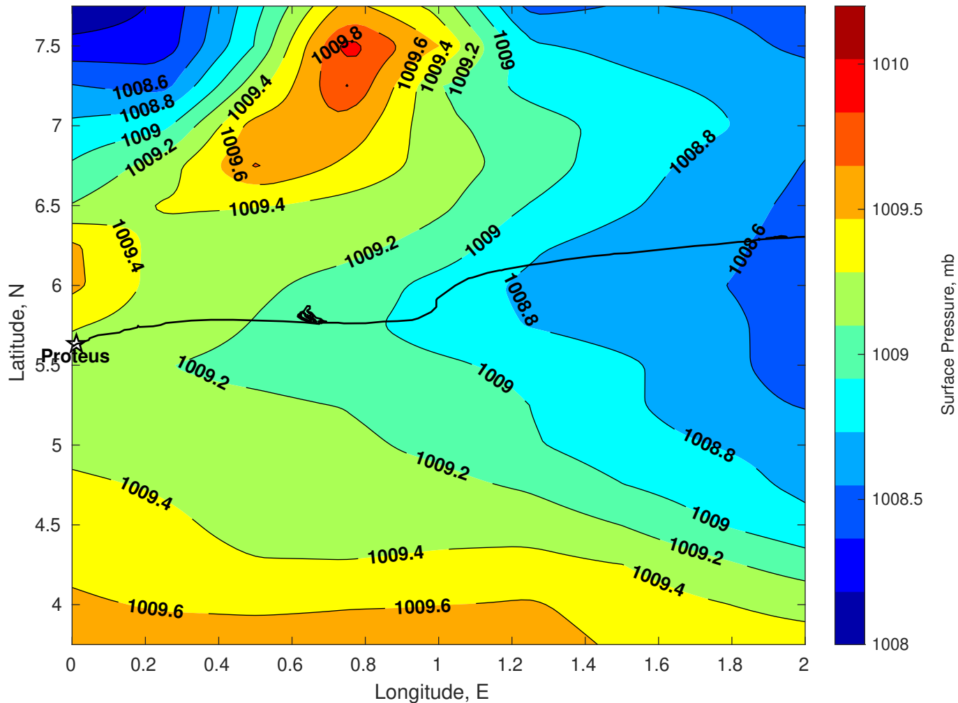
Surface Pressure (mb) for Proteus at 03-Dec-2025 00:00:00
