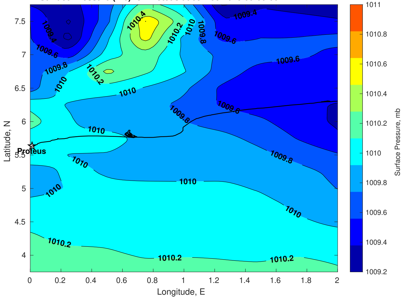
Surface Pressure (mb) for Proteus at 05-Dec-2025 00:00:00
