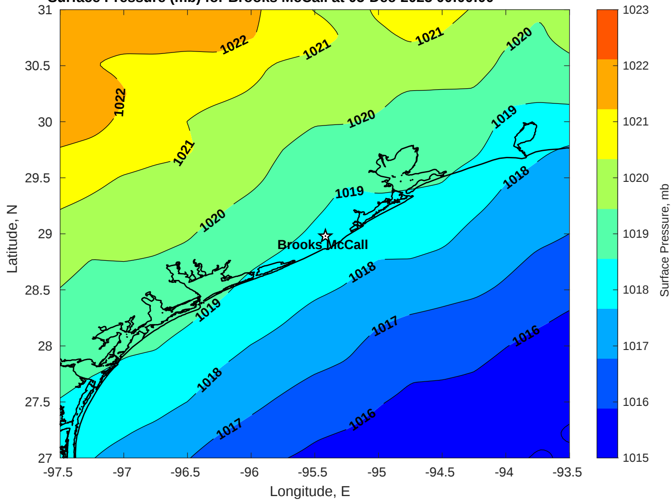
Surface Pressure (mb) for Brooks McCall at 05-Dec-2025 00:00:00
