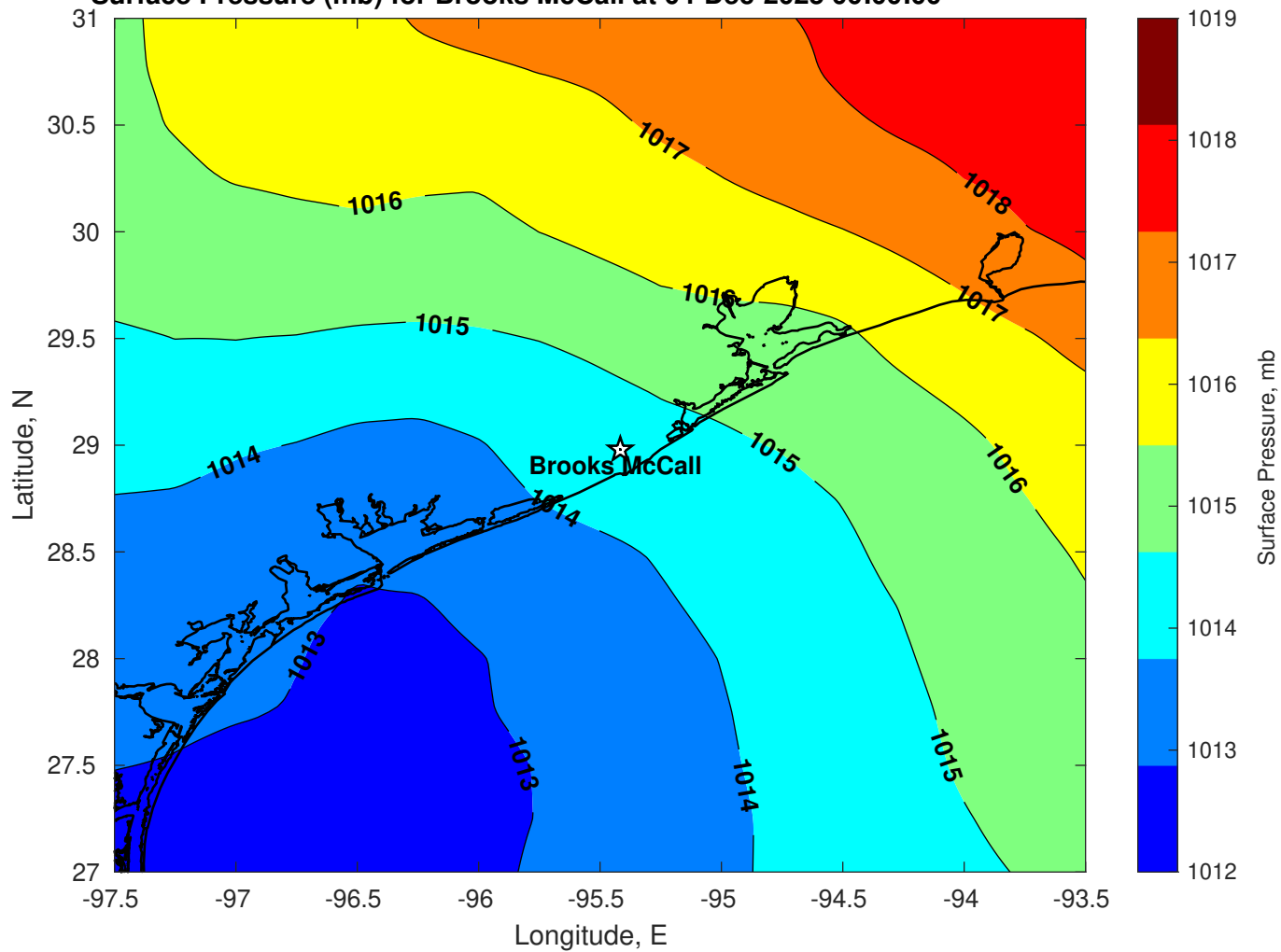
Surface Pressure (mb) for Brooks McCall at 04-Dec-2025 00:00:00
