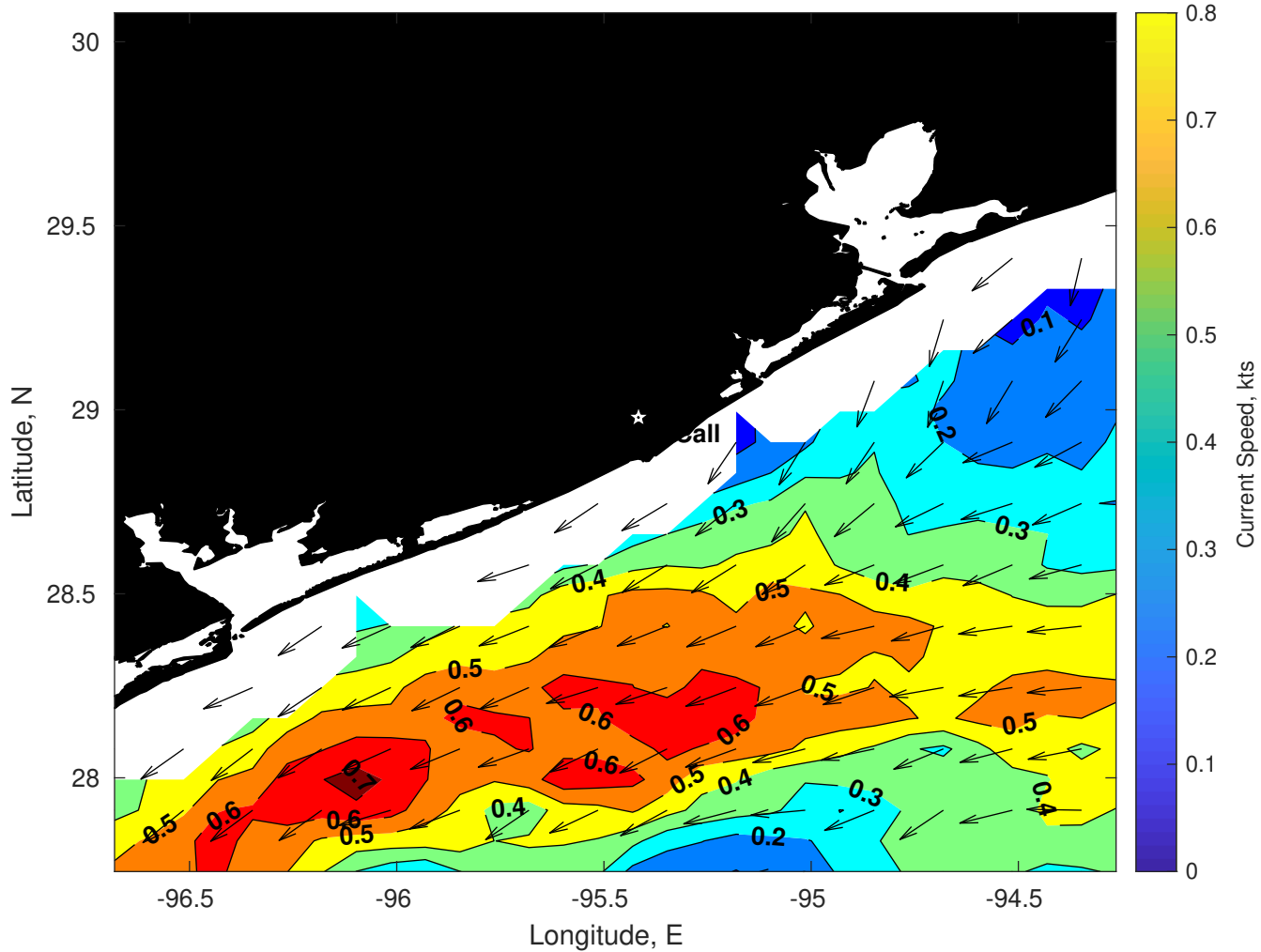
Surface Currents for Brooks McCall at 03-Dec-2025 00:00:00
