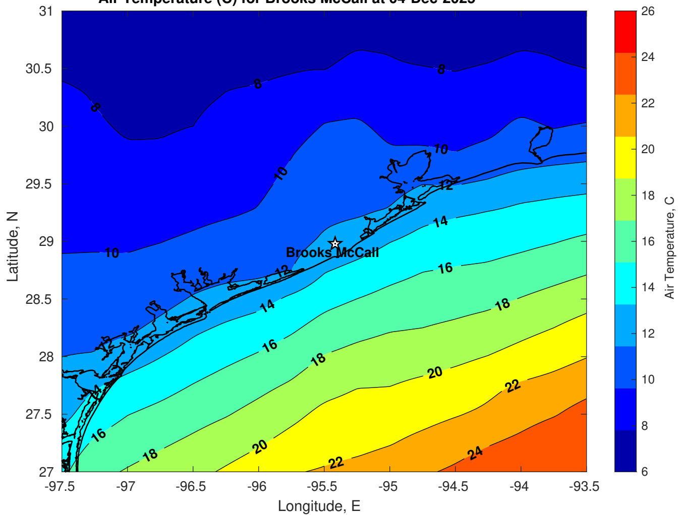
Air Temperature (C) for Brooks McCall at 04-Dec-2025
