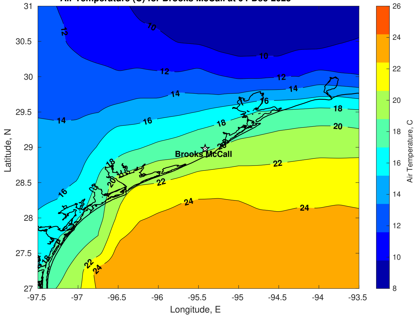
Air Temperature (C) for Brooks McCall at 04-Dec-2025
