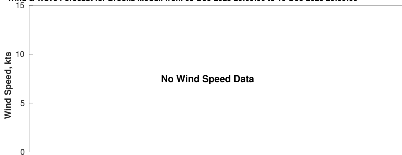
Wind & Wave Forecast for Brooks McCall from 03-Dec-2025 20:00:00 to 19-Dec-2025 20:00:00
