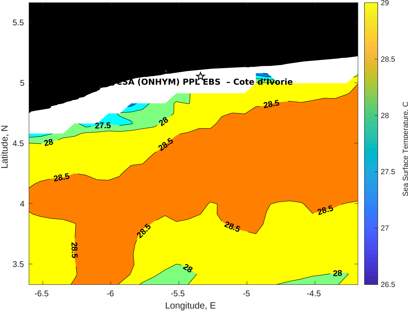
SST for CSA (ONHYM) PPL EBS - Cote d'Ivoire at 03-Dec-2025 00:00:00
