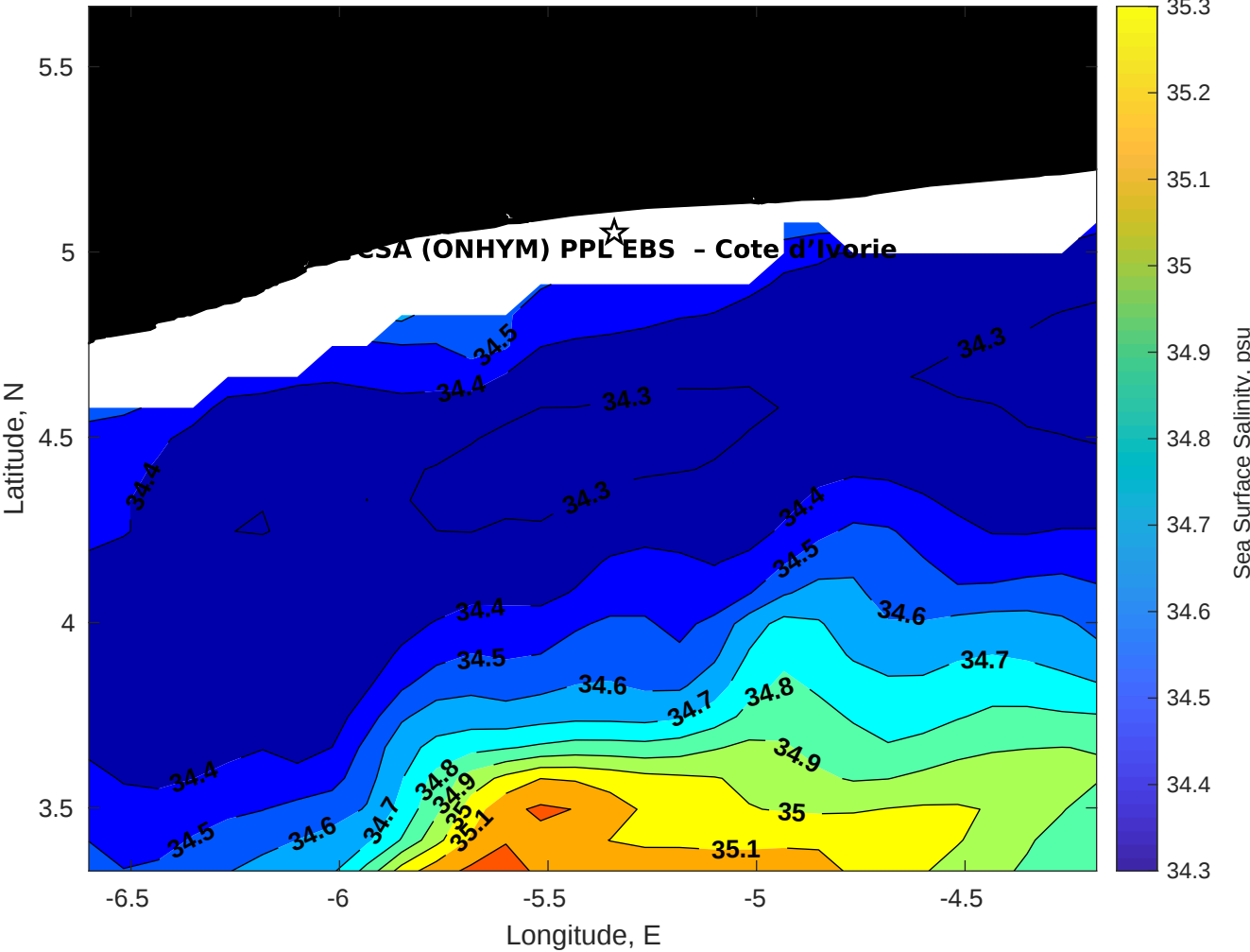
Surface Salinity for CSA (ONHYM) PPL EBS - Cote d'Ivoire at 03-Dec-2025 00:00:00
