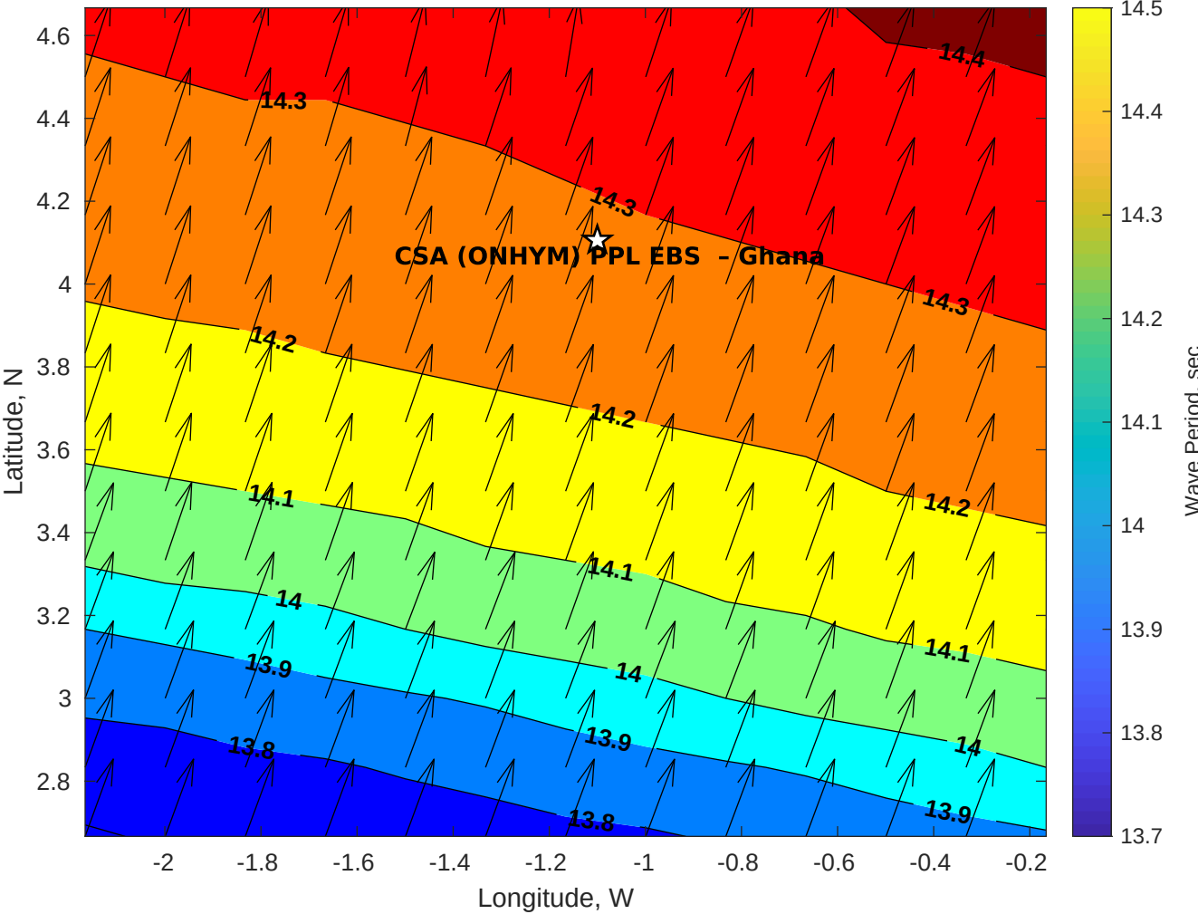
GFS Wave Period (sec) for CSA (ONHYM) PPL EBS - Ghana at 04-Dec-2025 09:00:00
