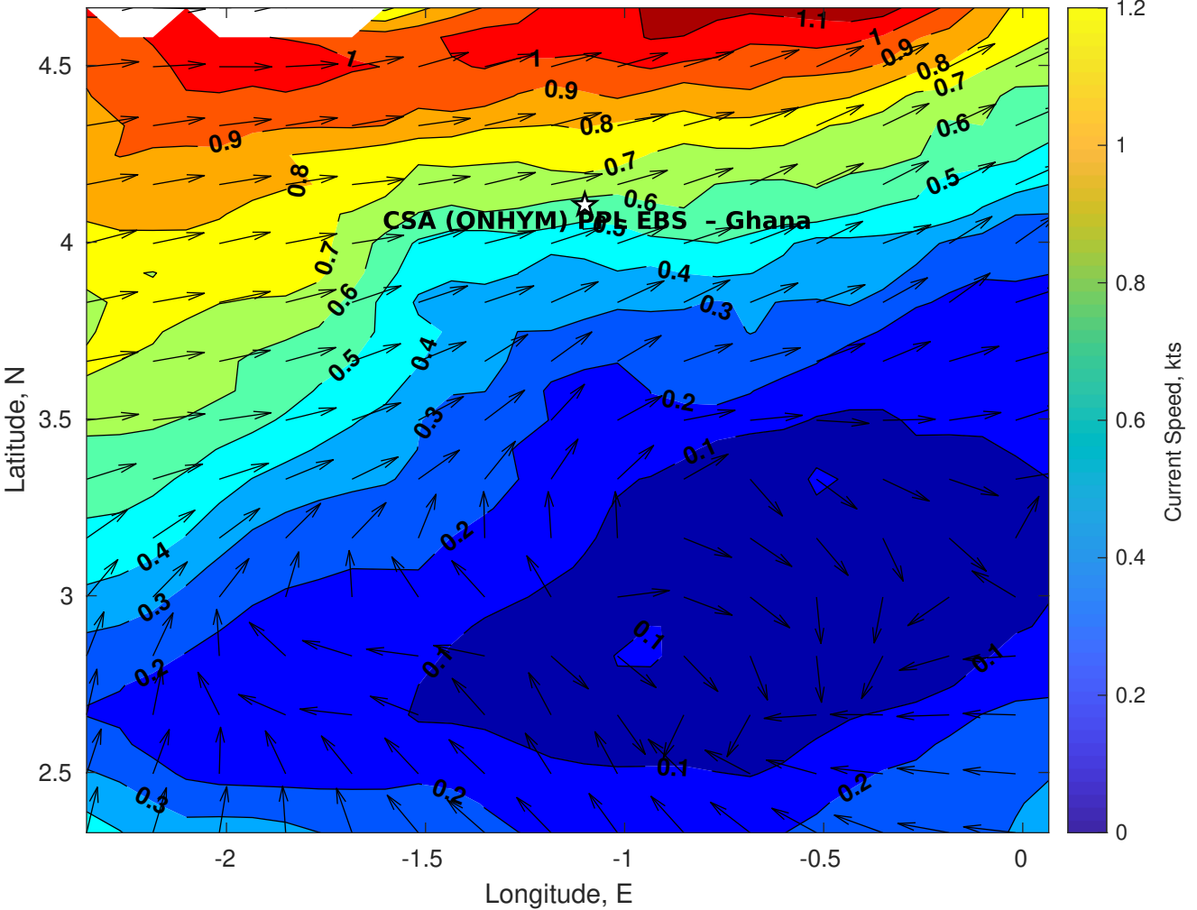
Surface Currents for CSA (ONHYM) PPL EBS - Ghana at 03-Dec-2025 00:00:00
