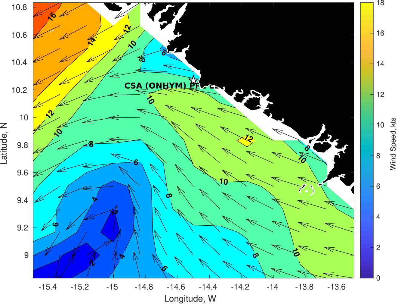
GFS Winds (kts) for CSA (ONHYM) PPL EBS - Guinea at 04-Dec-2025 09:00:00
