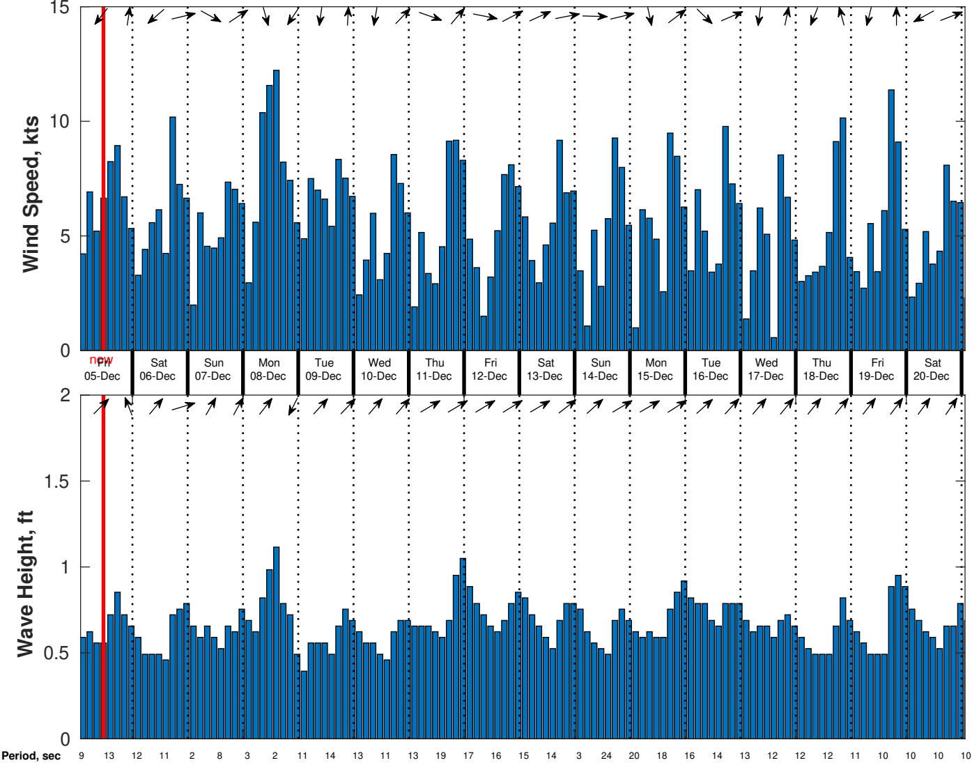
Wind & Wave Forecast for CSA (ONHYM) PPL EBS - Guinea from 04-Dec-2025 01:00:00 to 20-Dec-2025 01:00:00
