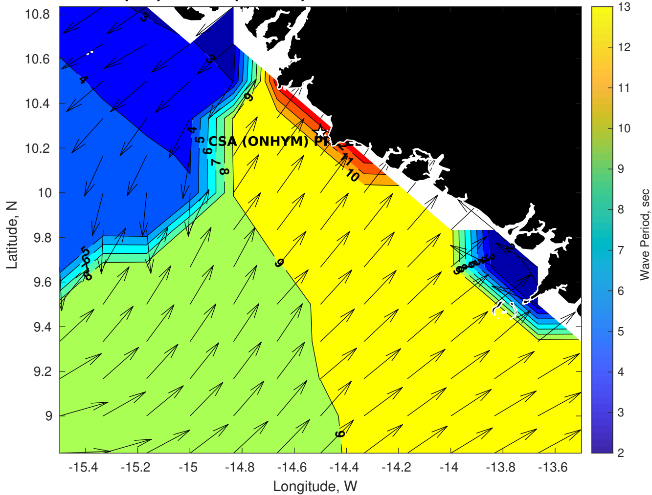
GFS Wave Period (sec) for CSA (ONHYM) PPL EBS - Guinea at 04-Dec-2025 09:00:00
