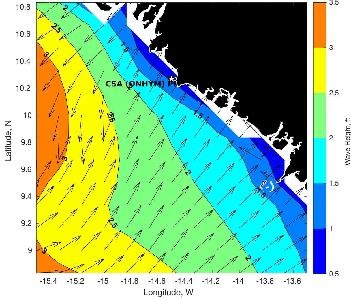
GFS Wave Height (ft) for CSA (ONHYM) PPL EBS - Guinea at 04-Dec-2025 09:00:00
