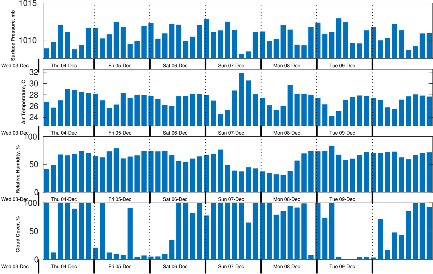
Met Forecast for CSA (ONHYM) PPL EBS - Guinea from 04-Dec-2025 00:00:00 to 11-Dec-2025 00:00:00
