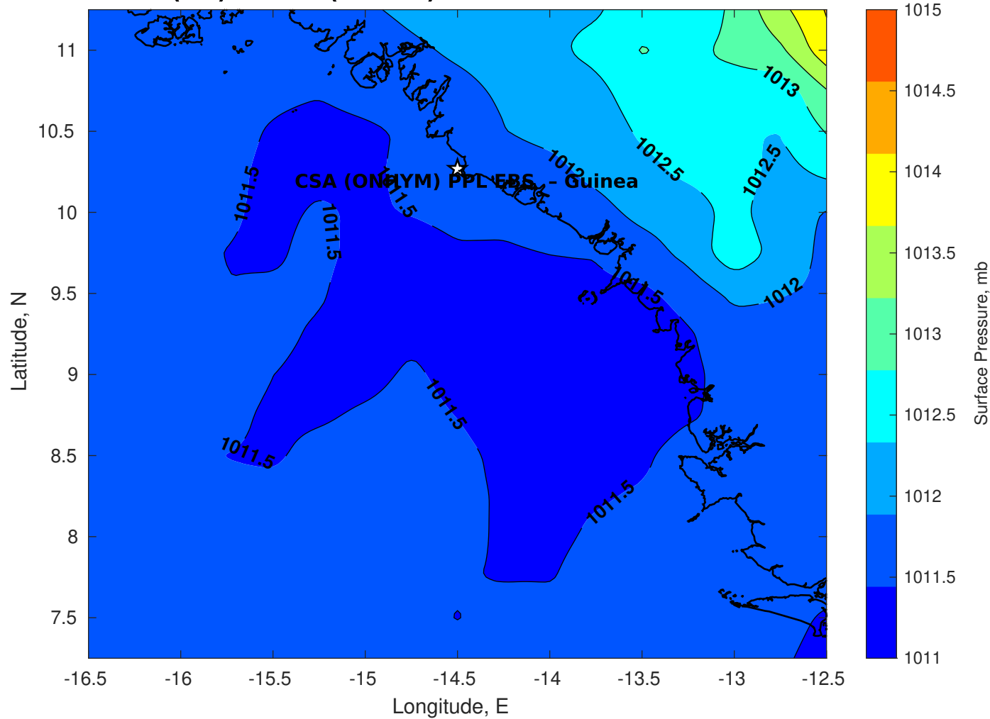
Surface Pressure (mb) for CSA (ONHYM) PPL EBS - Guinea at 05-Dec-2025 00:00:00
