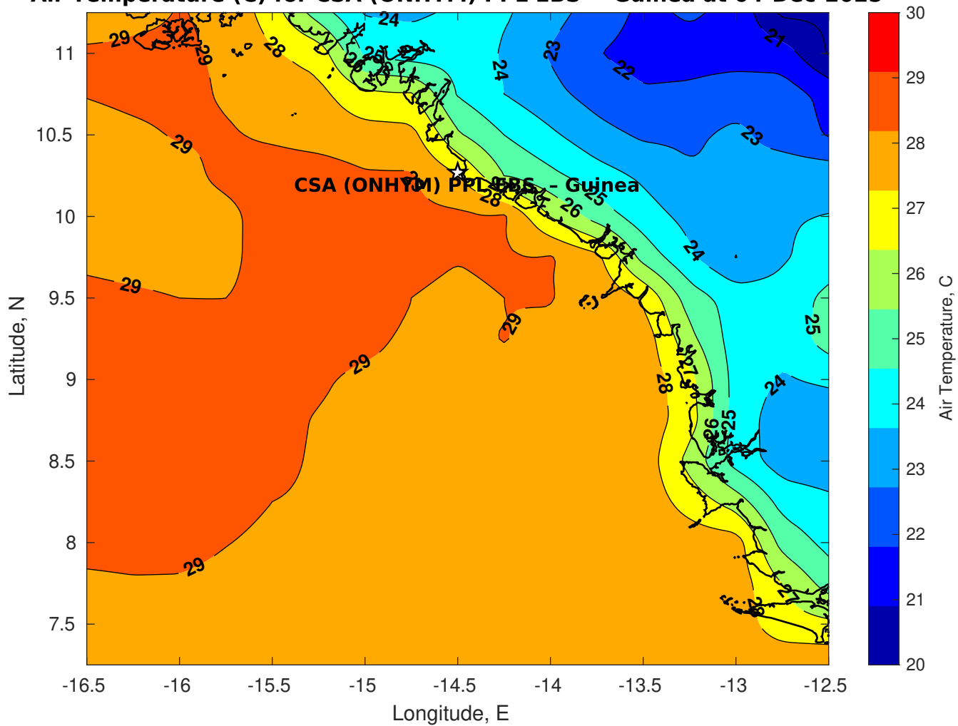
Air Temperature (C) for CSA (ONHYM) PPL EBS - Guinea at 04-Dec-2025
