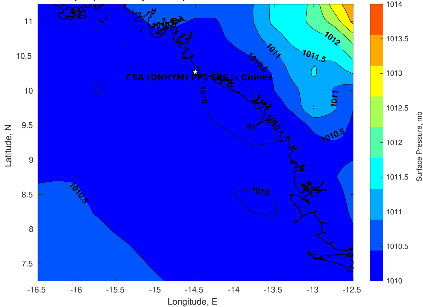
Surface Pressure (mb) for CSA (ONHYM) PPL EBS - Guinea at 04-Dec-2025 00:00:00
