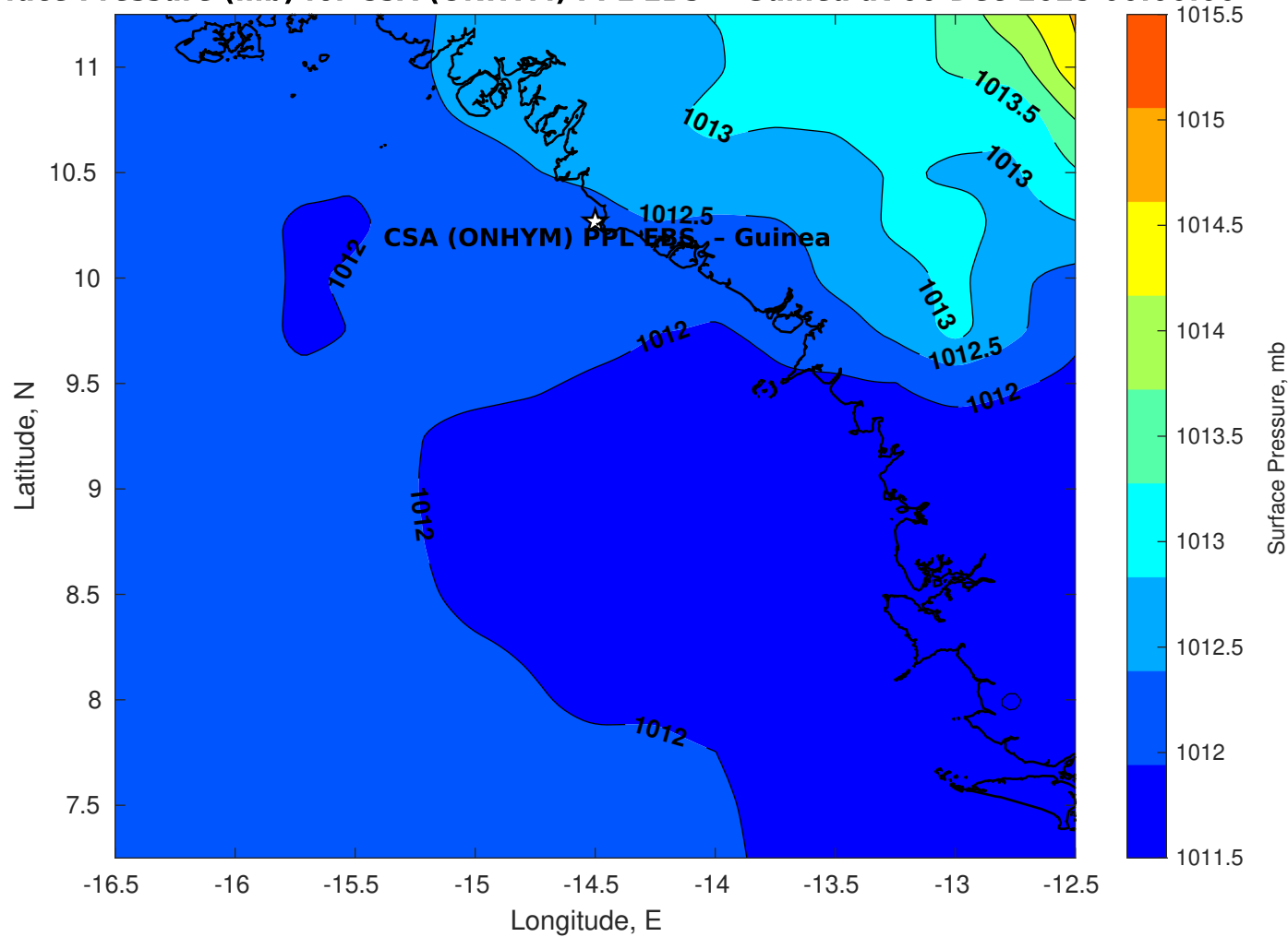
Surface Pressure (mb) for CSA (ONHYM) PPL EBS - Guinea at 06-Dec-2025 00:00:00
